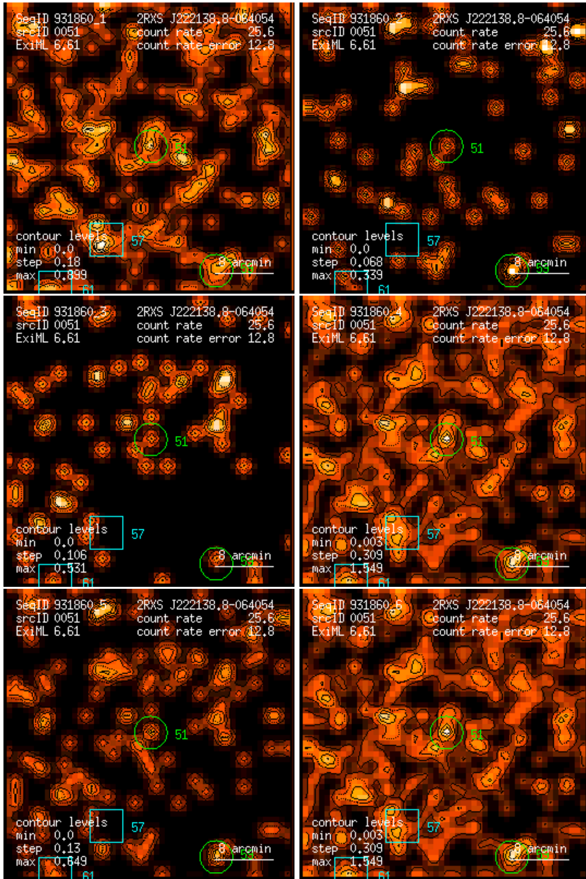
Figure 51: RASS 931860: detection 0051: band rate images, Gaussian filter: (1) PSPC channels 11 – 41, (2) 52 – 90, (3) 91 – 201, (4) 11 – 235, (5) 52 – 201, (6) 11 – 201. Broad band rates in counts/ks. Band rate contour levels in counts/ks/arcmin 2 .
