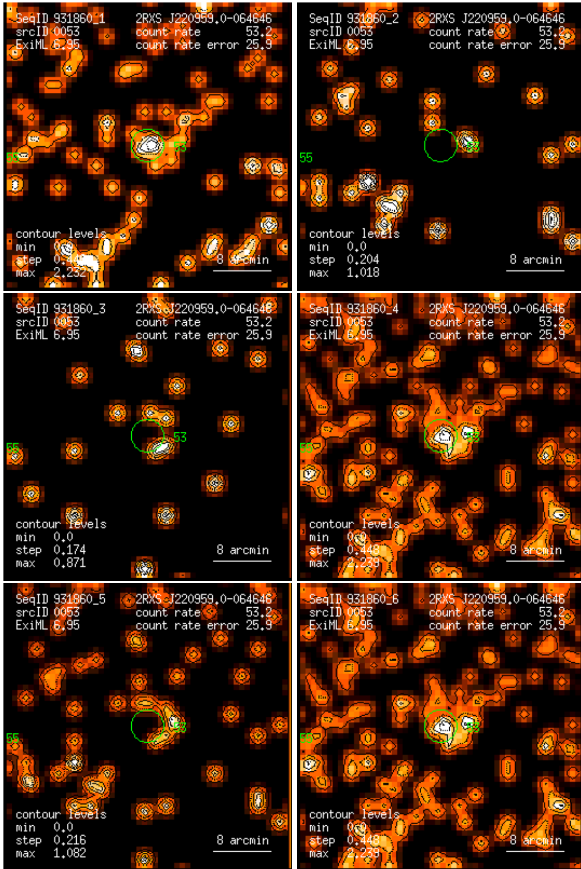
Figure 53: RASS 931860: detection 0053: band rate images, Gaussian filter: (1) PSPC channels 11 – 41, (2) 52 – 90, (3) 91 – 201, (4) 11 – 235, (5) 52 – 201, (6) 11 – 201. Broad band rates in counts/ks. Band rate contour levels in counts/ks/arcmin 2 .
