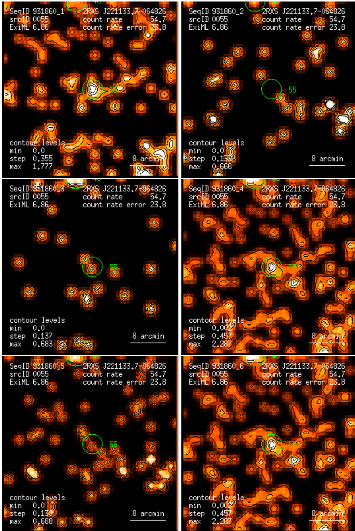
Figure 55: RASS 931860: detection 0055: band rate images, Gaussian filter: (1) PSPC channels 11 – 41, (2) 52 – 90, (3) 91 – 201, (4) 11 – 235, (5) 52 – 201, (6) 11 – 201. Broad band rates in counts/ks. Band rate contour levels in counts/ks/arcmin 2 .
