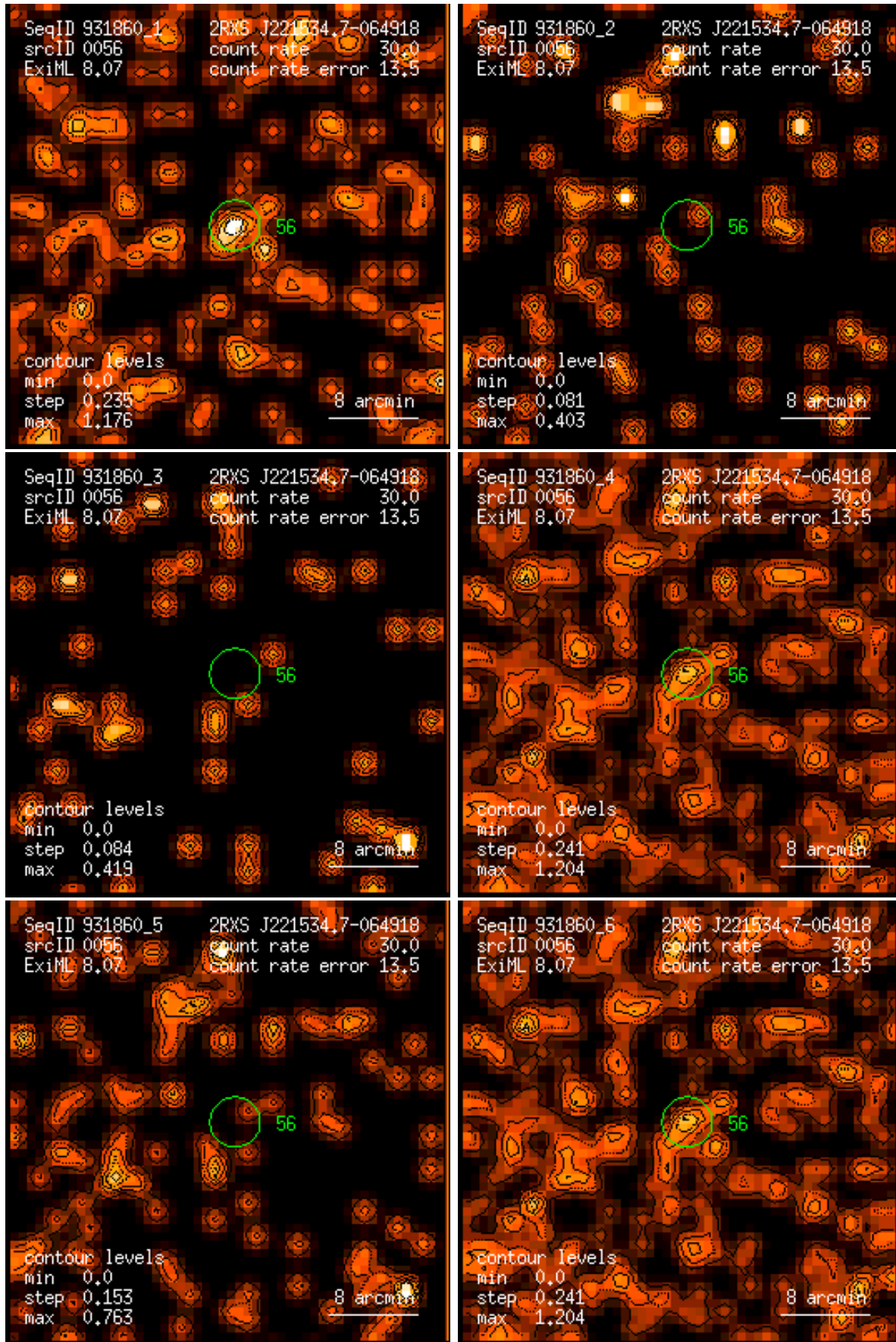
Figure 56: RASS 931860: detection 0056: band rate images, Gaussian filter: (1) PSPC channels 11 – 41, (2) 52 – 90, (3) 91 – 201, (4) 11 – 235, (5) 52 – 201, (6) 11 – 201. Broad band rates in counts/ks. Band rate contour levels in counts/ks/arcmin 2 .
