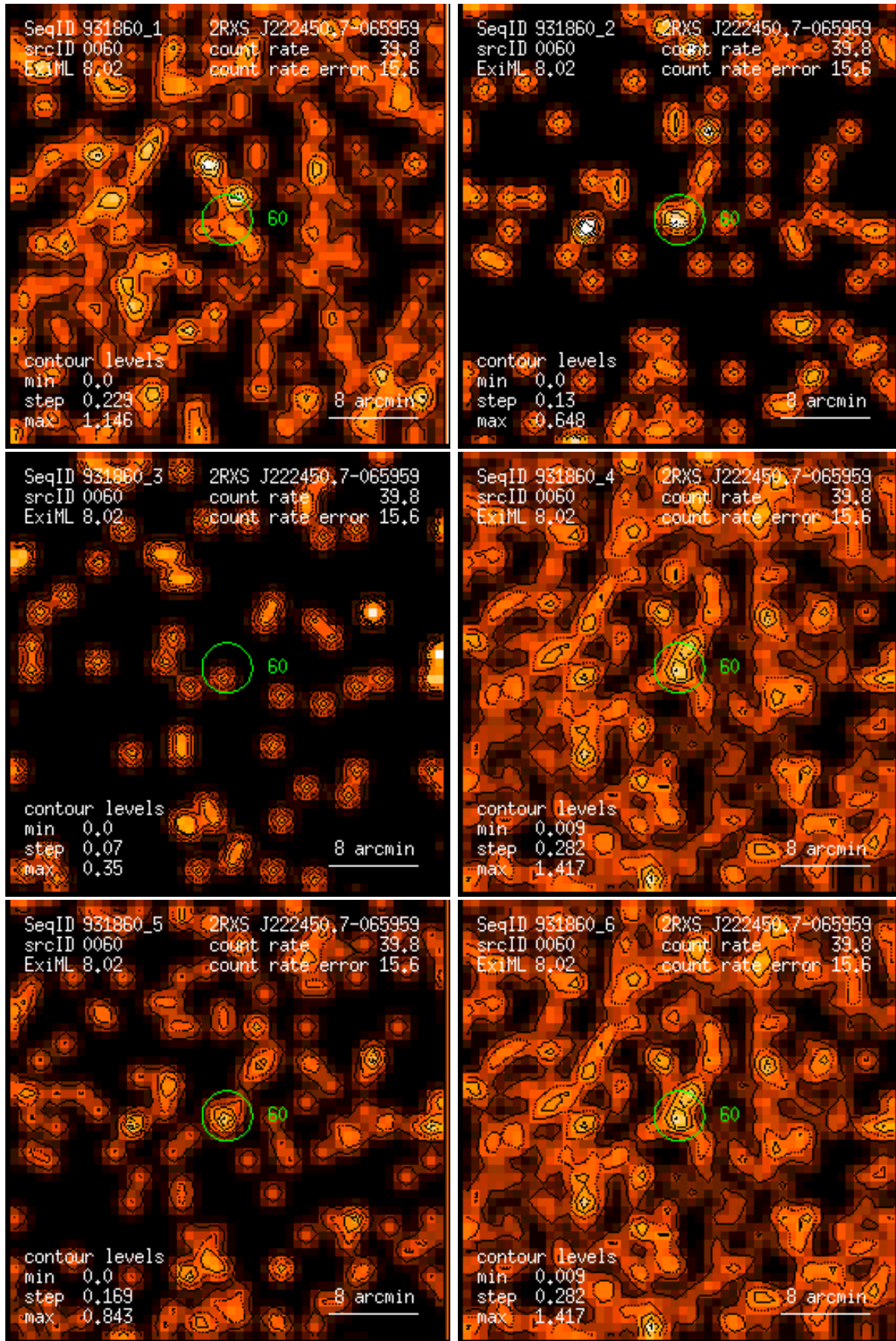
Figure 60: RASS 931860: detection 0060: band rate images, Gaussian filter: (1) PSPC channels 11 – 41, (2) 52 – 90, (3) 91 – 201, (4) 11 – 235, (5) 52 – 201, (6) 11 – 201. Broad band rates in counts/ks. Band rate contour levels in counts/ks/arcmin 2 .
