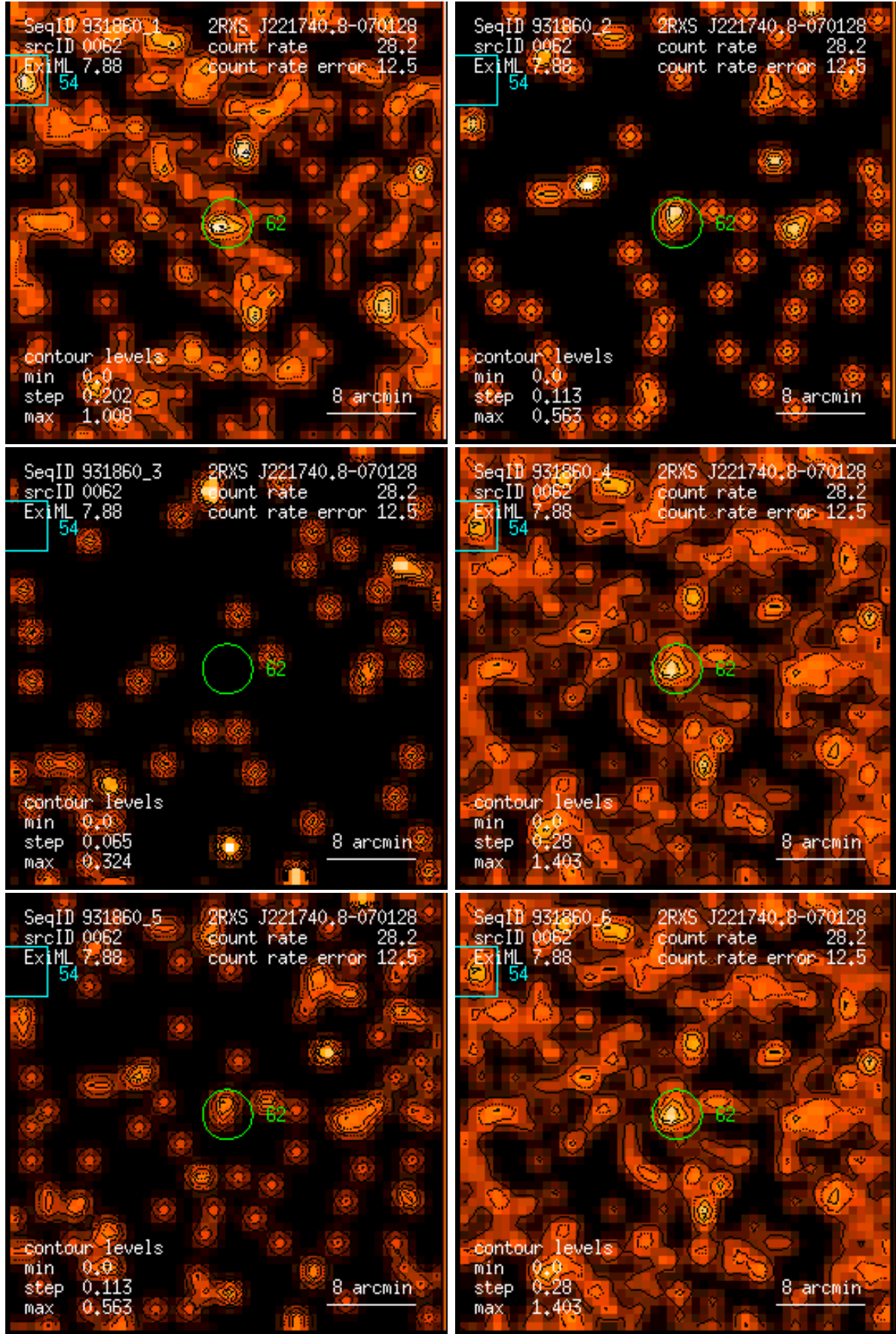
Figure 62: RASS 931860: detection 0062: band rate images, Gaussian filter: (1) PSPC channels 11 – 41, (2) 52 – 90, (3) 91 – 201, (4) 11 – 235, (5) 52 – 201, (6) 11 – 201. Broad band rates in counts/ks. Band rate contour levels in counts/ks/arcmin 2 .
