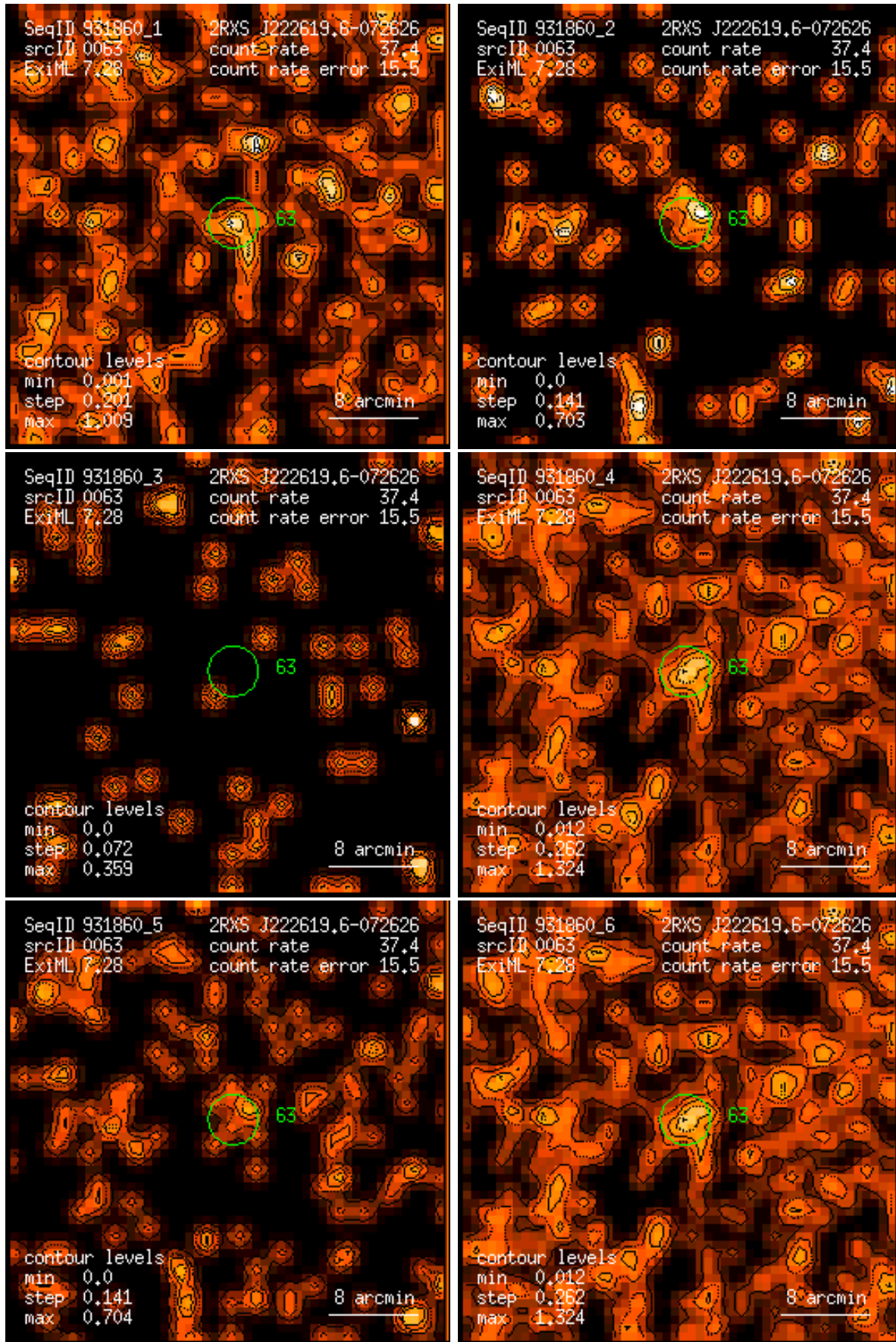
Figure 63: RASS 931860: detection 0063: band rate images, Gaussian filter: (1) PSPC channels 11 – 41, (2) 52 – 90, (3) 91 – 201, (4) 11 – 235, (5) 52 – 201, (6) 11 – 201. Broad band rates in counts/ks. Band rate contour levels in counts/ks/arcmin 2 .
