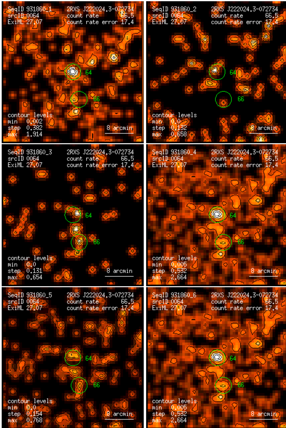
Figure 64: RASS 931860: detection 0064: band rate images, Gaussian filter: (1) PSPC channels 11 – 41, (2) 52 – 90, (3) 91 – 201, (4) 11 – 235, (5) 52 – 201, (6) 11 – 201. Broad band rates in counts/ks. Band rate contour levels in counts/ks/arcmin 2 .
