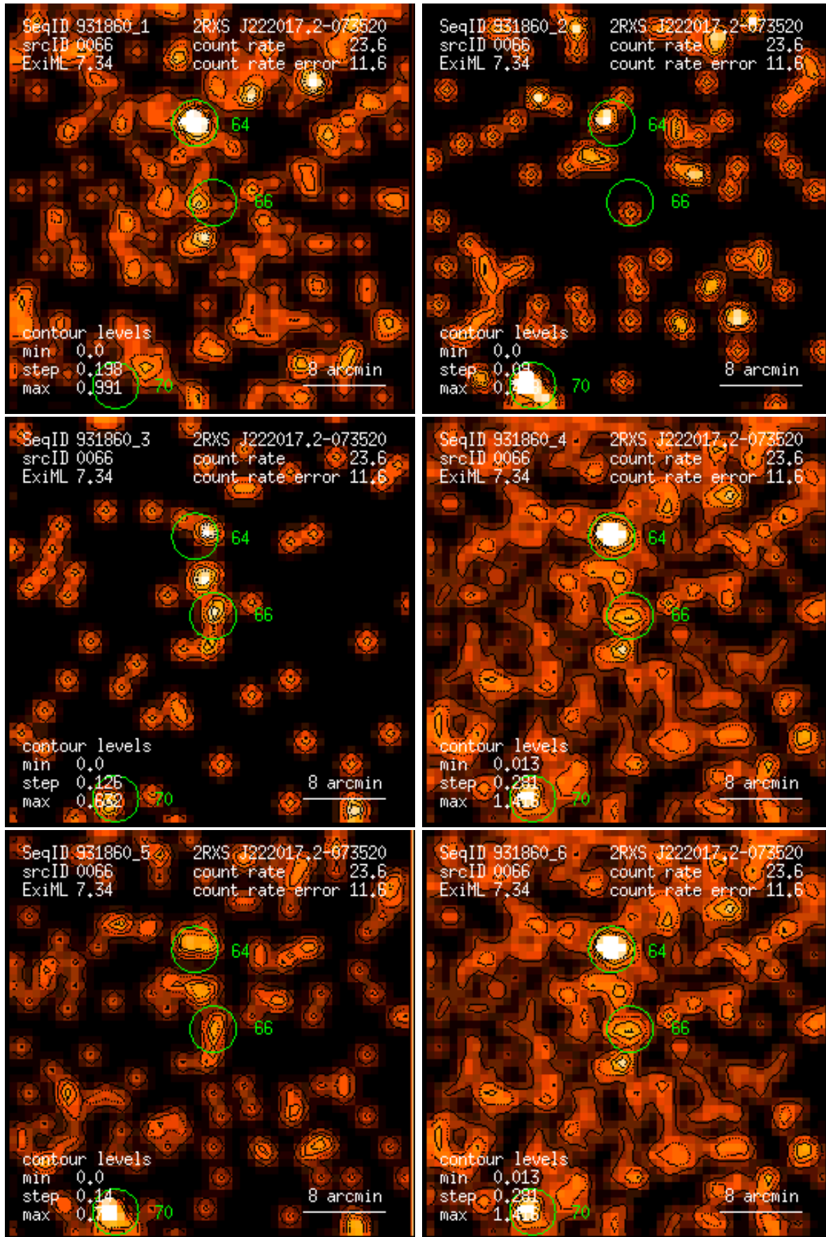
Figure 66: RASS 931860: detection 0066: band rate images, Gaussian filter: (1) PSPC channels 11 – 41, (2) 52 – 90, (3) 91 – 201, (4) 11 – 235, (5) 52 – 201, (6) 11 – 201. Broad band rates in counts/ks. Band rate contour levels in counts/ks/arcmin 2 .
