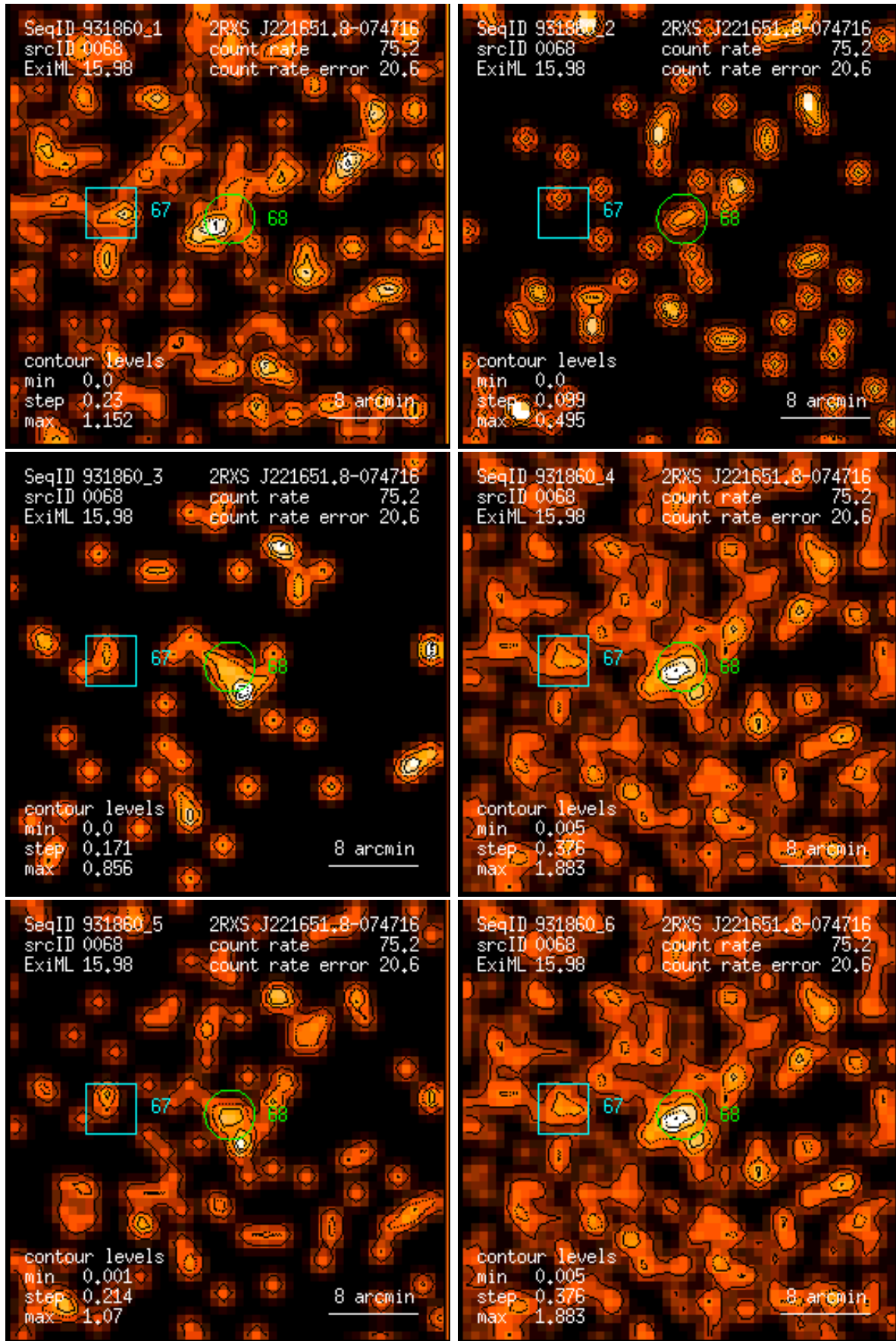
Figure 68: RASS 931860: detection 0068: band rate images, Gaussian filter: (1) PSPC channels 11 – 41, (2) 52 – 90, (3) 91 – 201, (4) 11 – 235, (5) 52 – 201, (6) 11 – 201. Broad band rates in counts/ks. Band rate contour levels in counts/ks/arcmin 2 .
