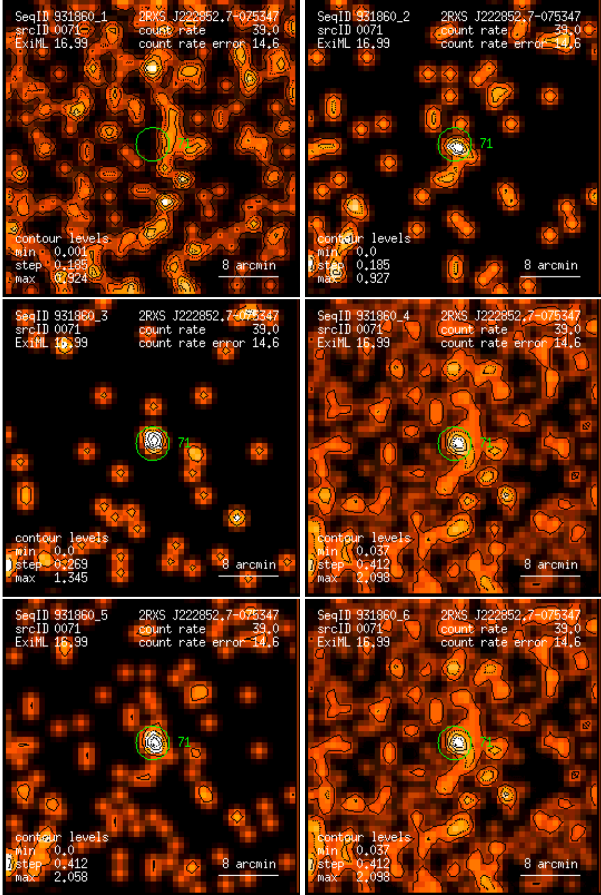
Figure 71: RASS 931860: detection 0071: band rate images, Gaussian filter: (1) PSPC channels 11 – 41, (2) 52 – 90, (3) 91 – 201, (4) 11 – 235, (5) 52 – 201, (6) 11 – 201. Broad band rates in counts/ks. Band rate contour levels in counts/ks/arcmin 2 .
