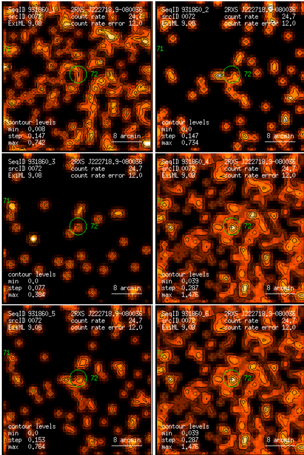
Figure 72: RASS 931860: detection 0072: band rate images, Gaussian filter: (1) PSPC channels 11 – 41, (2) 52 – 90, (3) 91 – 201, (4) 11 – 235, (5) 52 – 201, (6) 11 – 201. Broad band rates in counts/ks. Band rate contour levels in counts/ks/arcmin 2 .
