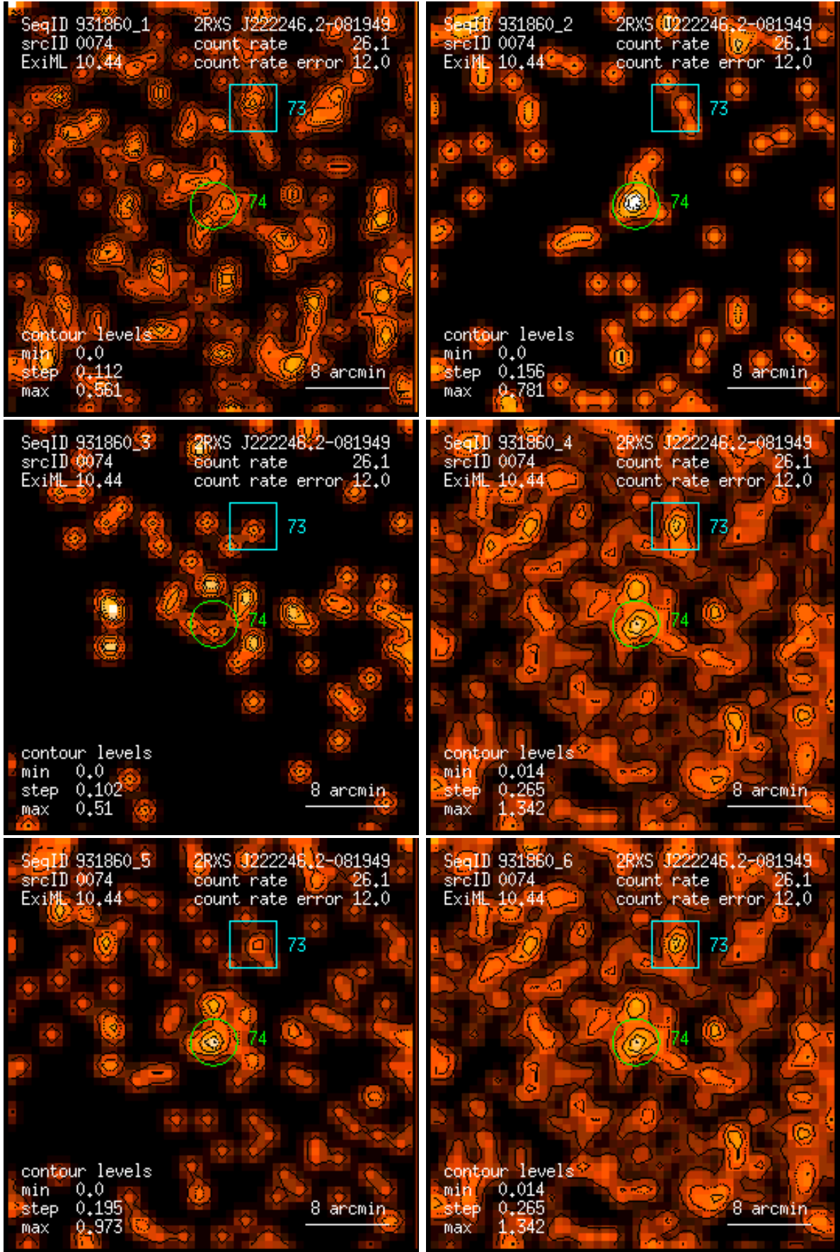
Figure 74: RASS 931860: detection 0074: band rate images, Gaussian filter: (1) PSPC channels 11 – 41, (2) 52 – 90, (3) 91 – 201, (4) 11 – 235, (5) 52 – 201, (6) 11 – 201. Broad band rates in counts/ks. Band rate contour levels in counts/ks/arcmin 2 .
