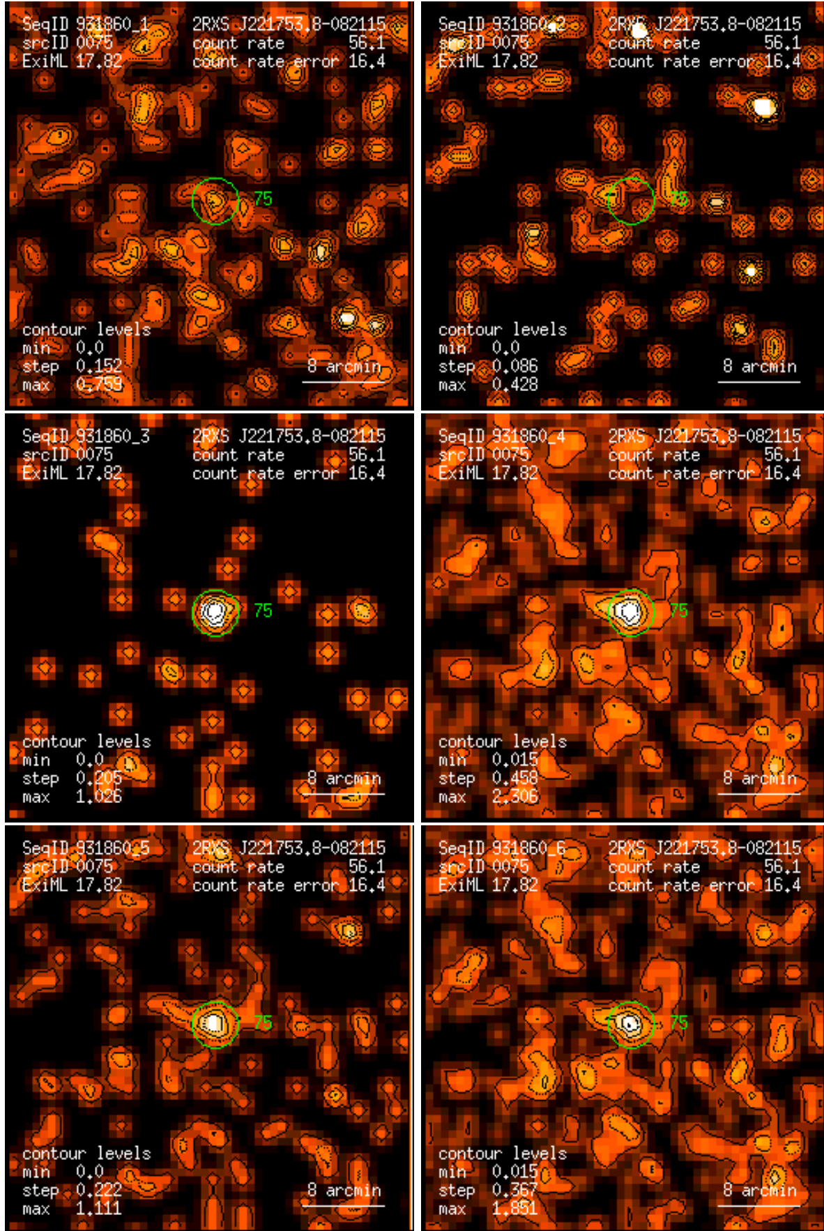
Figure 75: RASS 931860: detection 0075: band rate images, Gaussian filter: (1) PSPC channels 11 – 41, (2) 52 – 90, (3) 91 – 201, (4) 11 – 235, (5) 52 – 201, (6) 11 – 201. Broad band rates in counts/ks. Band rate contour levels in counts/ks/arcmin 2 .
