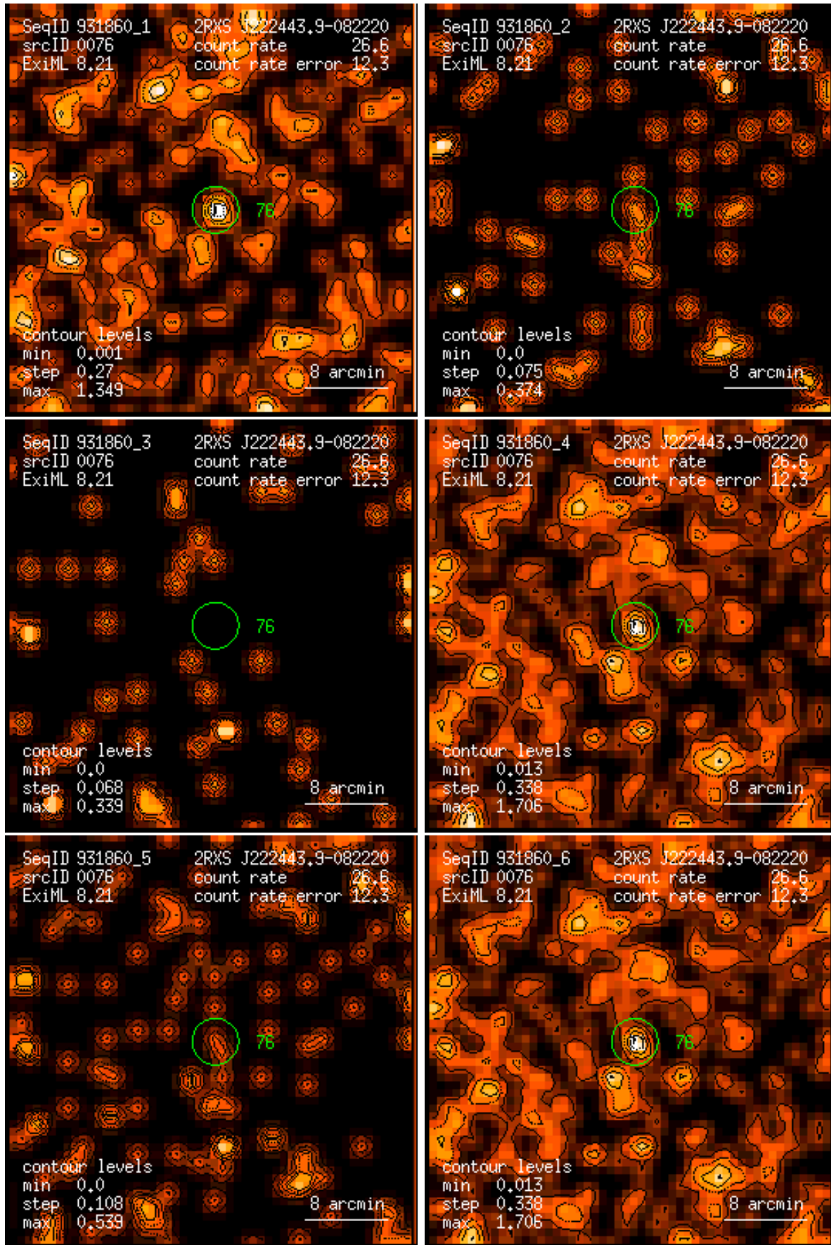
Figure 76: RASS 931860: detection 0076: band rate images, Gaussian filter: (1) PSPC channels 11 – 41, (2) 52 – 90, (3) 91 – 201, (4) 11 – 235, (5) 52 – 201, (6) 11 – 201. Broad band rates in counts/ks. Band rate contour levels in counts/ks/arcmin 2 .
