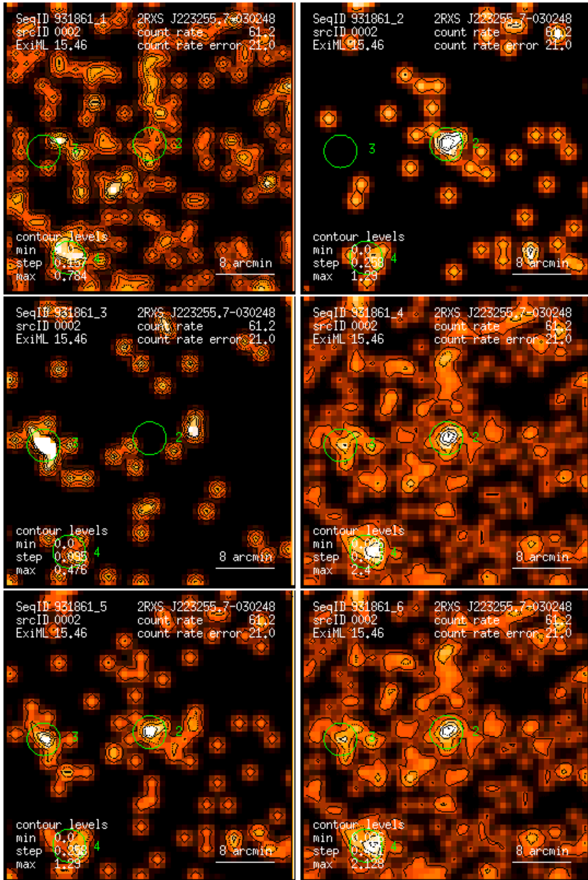
Figure 2: RASS 931861: detection 0002: band rate images, Gaussian filter: (1) PSPC channels 11 – 41, (2) 52 – 90, (3) 91 – 201, (4) 11 – 235, (5) 52 – 201, (6) 11 – 201. Broad band rates in counts/ks. Band rate contour levels in counts/ks/arcmin 2 .
