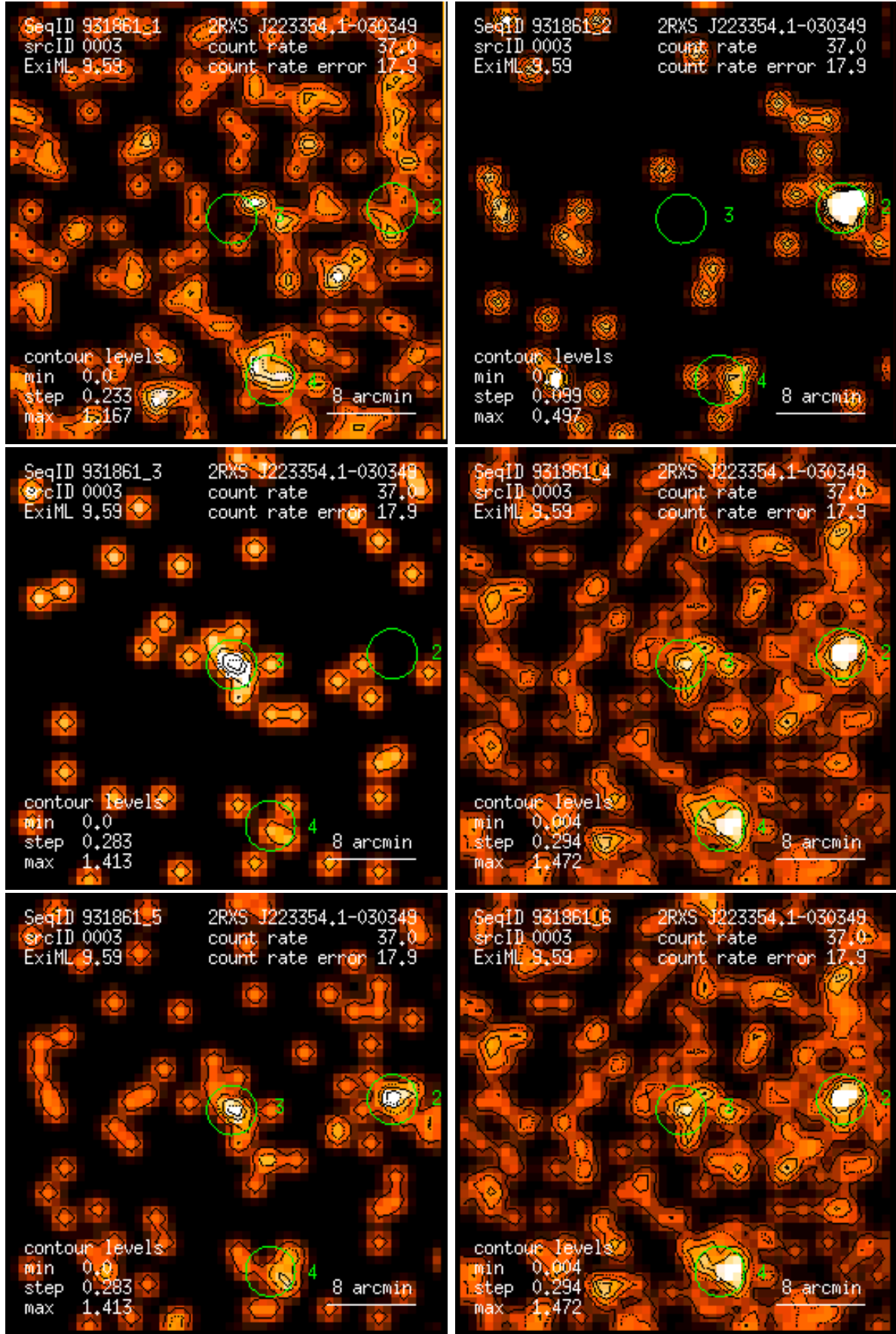
Figure 3: RASS 931861: detection 0003: band rate images, Gaussian filter: (1) PSPC channels 11 – 41, (2) 52 – 90, (3) 91 – 201, (4) 11 – 235, (5) 52 – 201, (6) 11 – 201. Broad band rates in counts/ks. Band rate contour levels in counts/ks/arcmin 2 .
