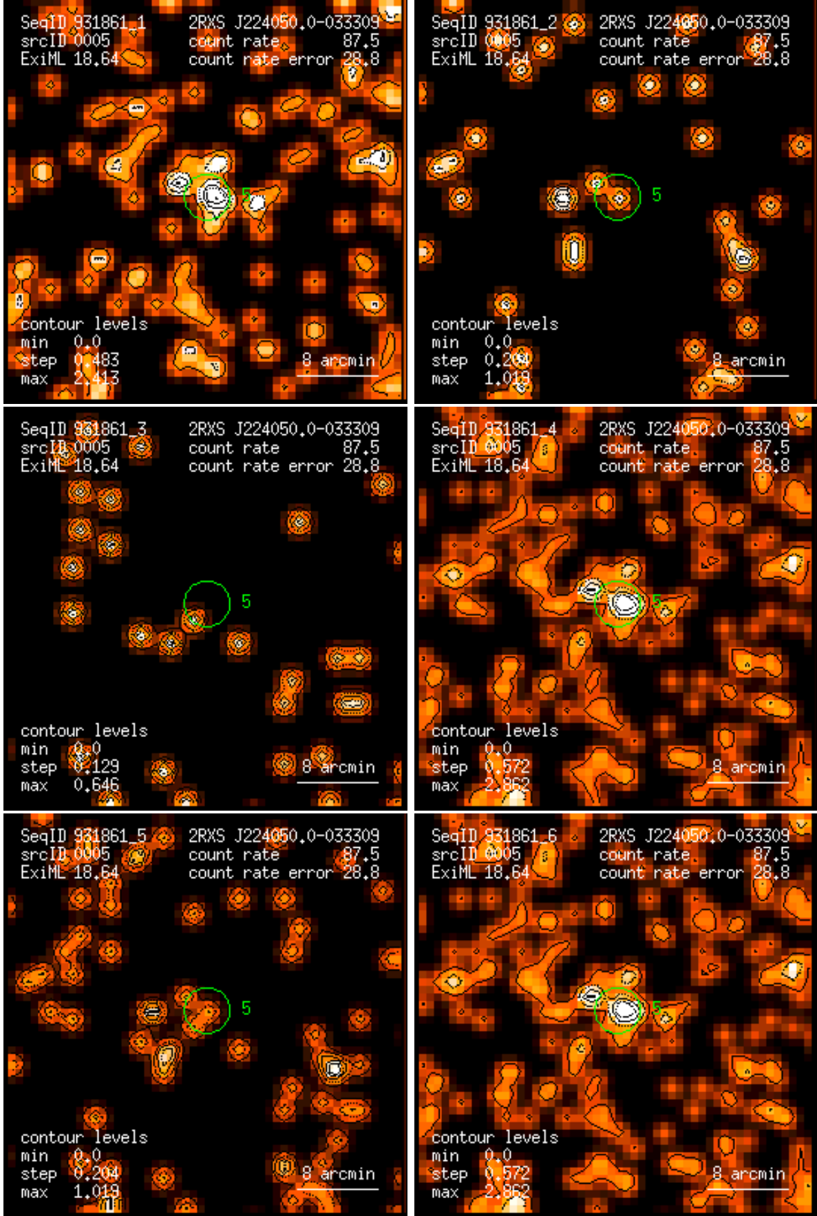
Figure 5: RASS 931861: detection 0005: band rate images, Gaussian filter: (1) PSPC channels 11 – 41, (2) 52 – 90, (3) 91 – 201, (4) 11 – 235, (5) 52 – 201, (6) 11 – 201. Broad band rates in counts/ks. Band rate contour levels in counts/ks/arcmin 2 .
