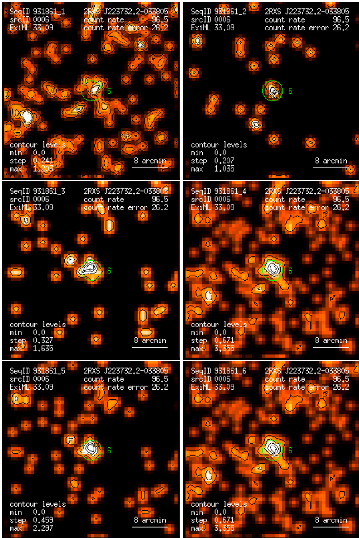
Figure 6: RASS 931861: detection 0006: band rate images, Gaussian filter: (1) PSPC channels 11 – 41, (2) 52 – 90, (3) 91 – 201, (4) 11 – 235, (5) 52 – 201, (6) 11 – 201. Broad band rates in counts/ks. Band rate contour levels in counts/ks/arcmin 2 .
