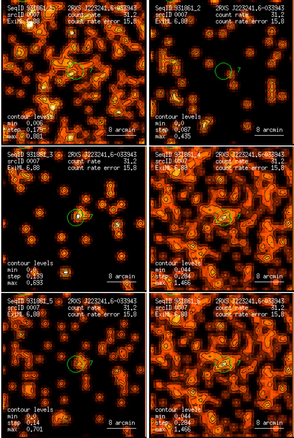
Figure 7: RASS 931861: detection 0007: band rate images, Gaussian filter: (1) PSPC channels 11 – 41, (2) 52 – 90, (3) 91 – 201, (4) 11 – 235, (5) 52 – 201, (6) 11 – 201. Broad band rates in counts/ks. Band rate contour levels in counts/ks/arcmin 2 .
