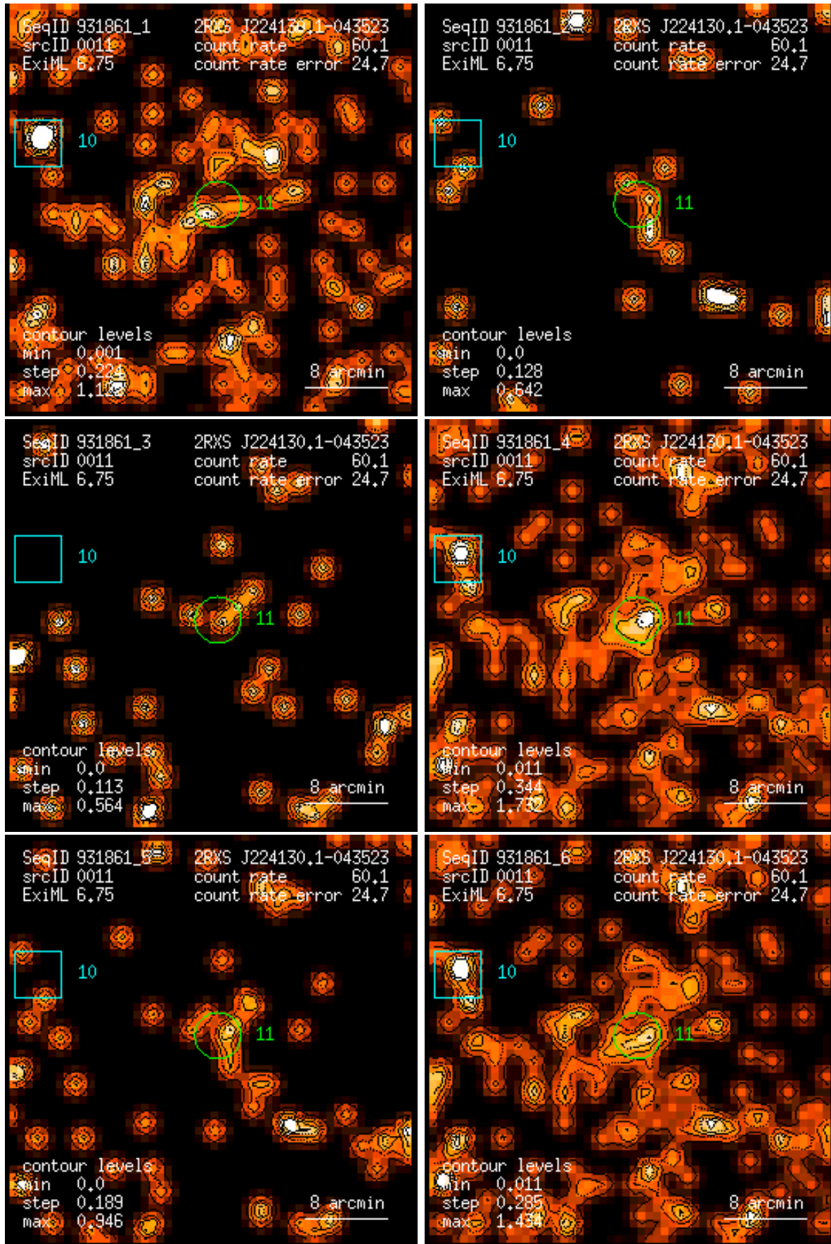
Figure 11: RASS 931861: detection 0011: band rate images, Gaussian filter: (1) PSPC channels 11 – 41, (2) 52 – 90, (3) 91 – 201, (4) 11 – 235, (5) 52 – 201, (6) 11 – 201. Broad band rates in counts/ks. Band rate contour levels in counts/ks/arcmin 2 .
