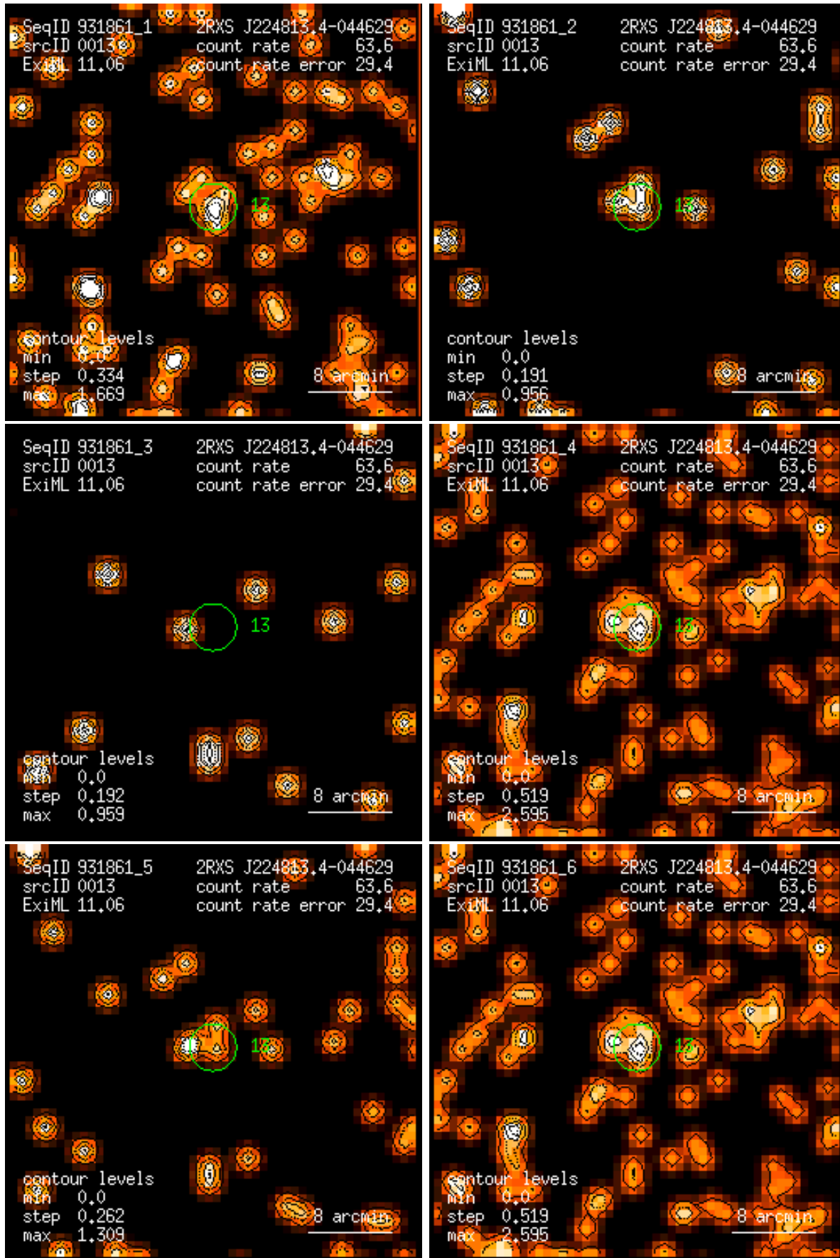
Figure 13: RASS 931861: detection 0013: band rate images, Gaussian filter: (1) PSPC channels 11 – 41, (2) 52 – 90, (3) 91 – 201, (4) 11 – 235, (5) 52 – 201, (6) 11 – 201. Broad band rates in counts/ks. Band rate contour levels in counts/ks/arcmin 2 .
