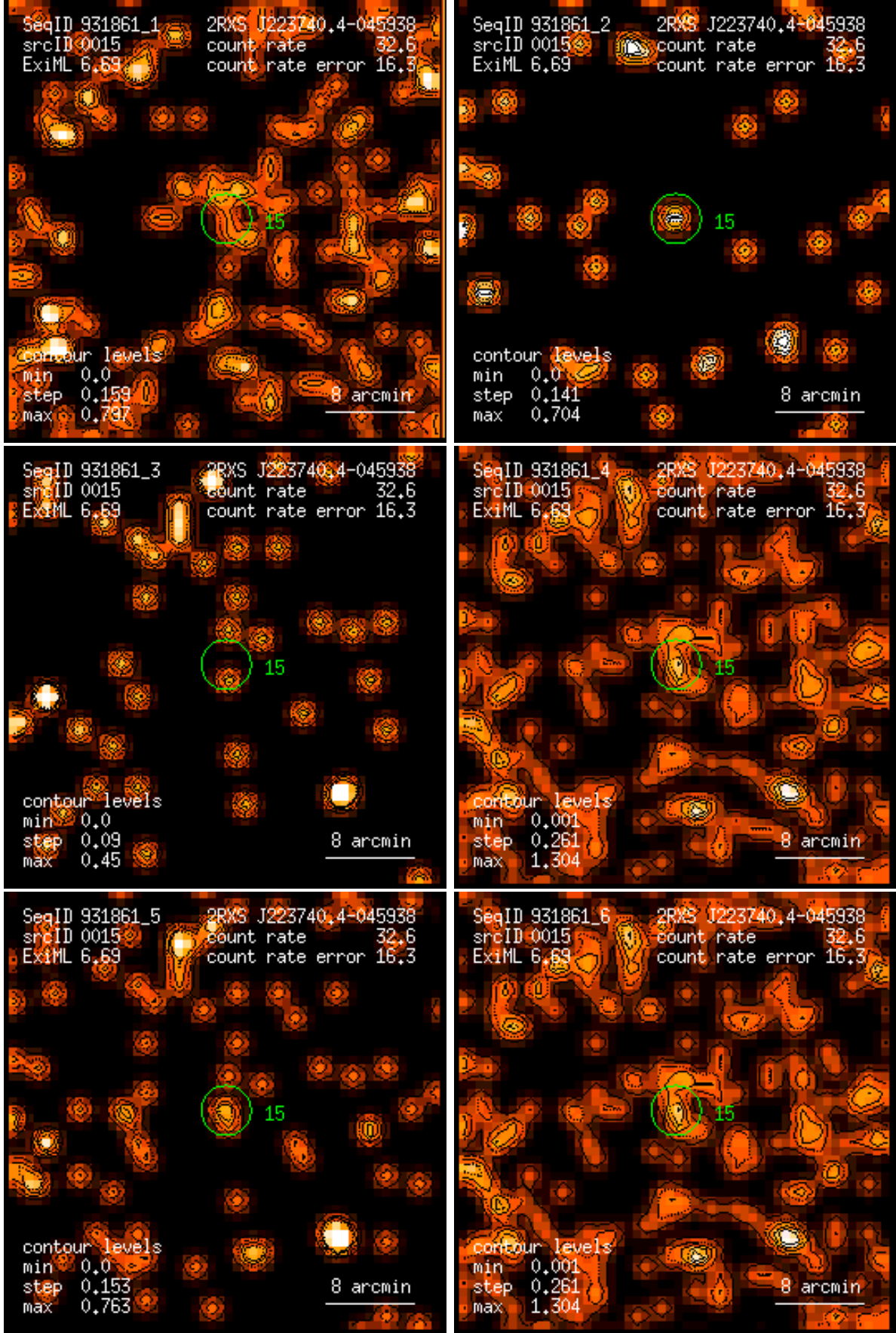
Figure 15: RASS 931861: detection 0015: band rate images, Gaussian filter: (1) PSPC channels 11 – 41, (2) 52 – 90, (3) 91 – 201, (4) 11 – 235, (5) 52 – 201, (6) 11 – 201. Broad band rates in counts/ks. Band rate contour levels in counts/ks/arcmin 2 .
