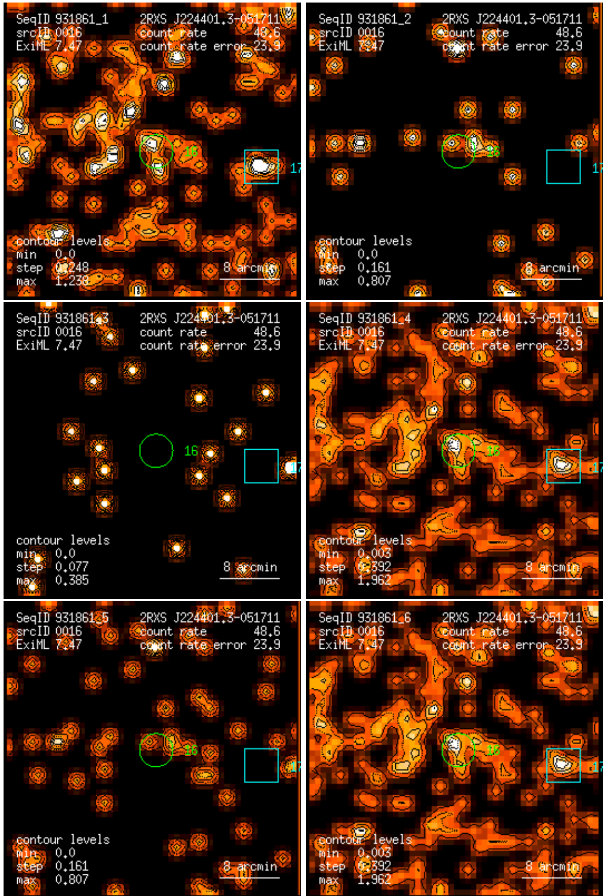
Figure 16: RASS 931861: detection 0016: band rate images, Gaussian filter: (1) PSPC channels 11 – 41, (2) 52 – 90, (3) 91 – 201, (4) 11 – 235, (5) 52 – 201, (6) 11 – 201. Broad band rates in counts/ks. Band rate contour levels in counts/ks/arcmin 2 .
