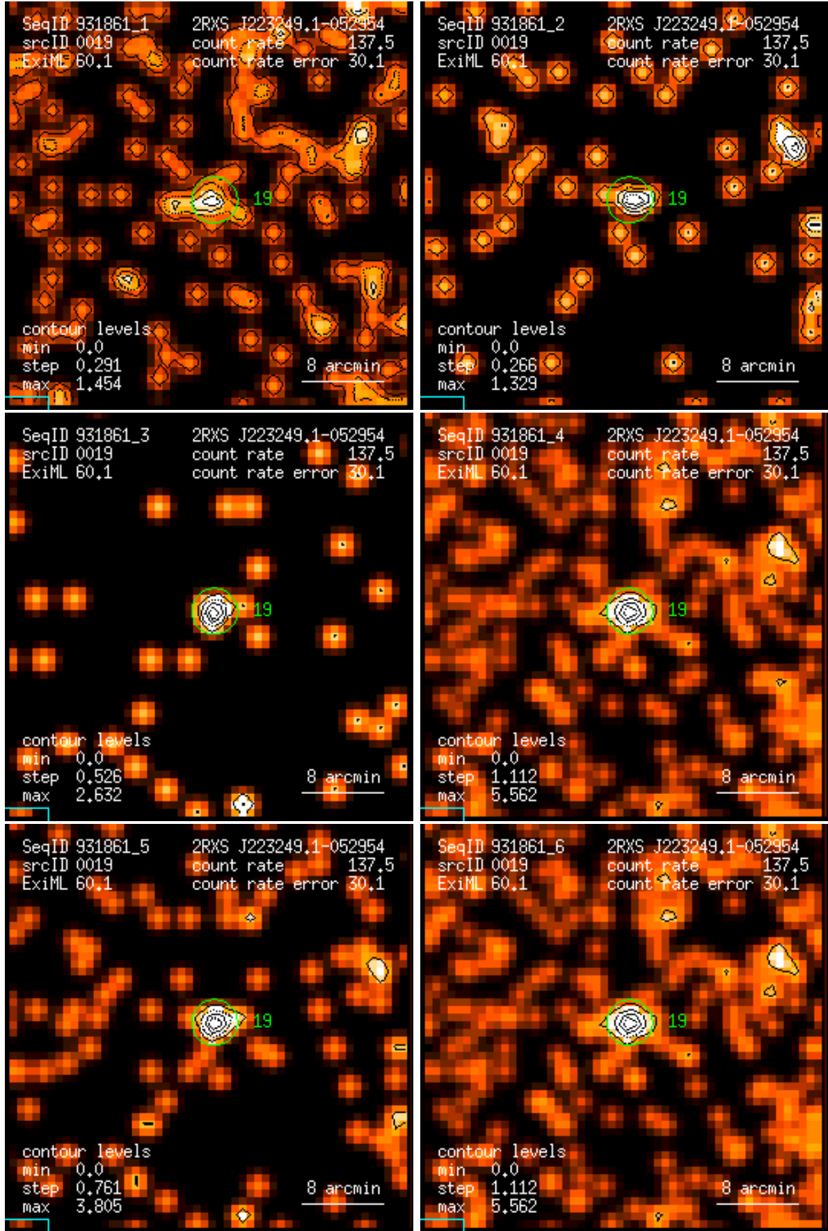
Figure 19: RASS 931861: detection 0019: band rate images, Gaussian filter: (1) PSPC channels 11 – 41, (2) 52 – 90, (3) 91 – 201, (4) 11 – 235, (5) 52 – 201, (6) 11 – 201. Broad band rates in counts/ks. Band rate contour levels in counts/ks/arcmin 2 .
