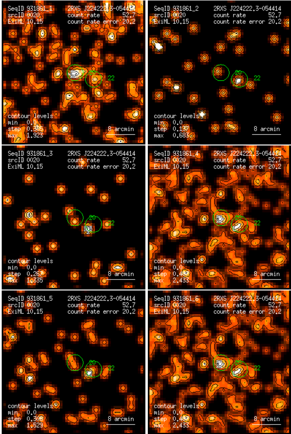
Figure 20: RASS 931861: detection 0020: band rate images, Gaussian filter: (1) PSPC channels 11 – 41, (2) 52 – 90, (3) 91 – 201, (4) 11 – 235, (5) 52 – 201, (6) 11 – 201. Broad band rates in counts/ks. Band rate contour levels in counts/ks/arcmin 2 .
