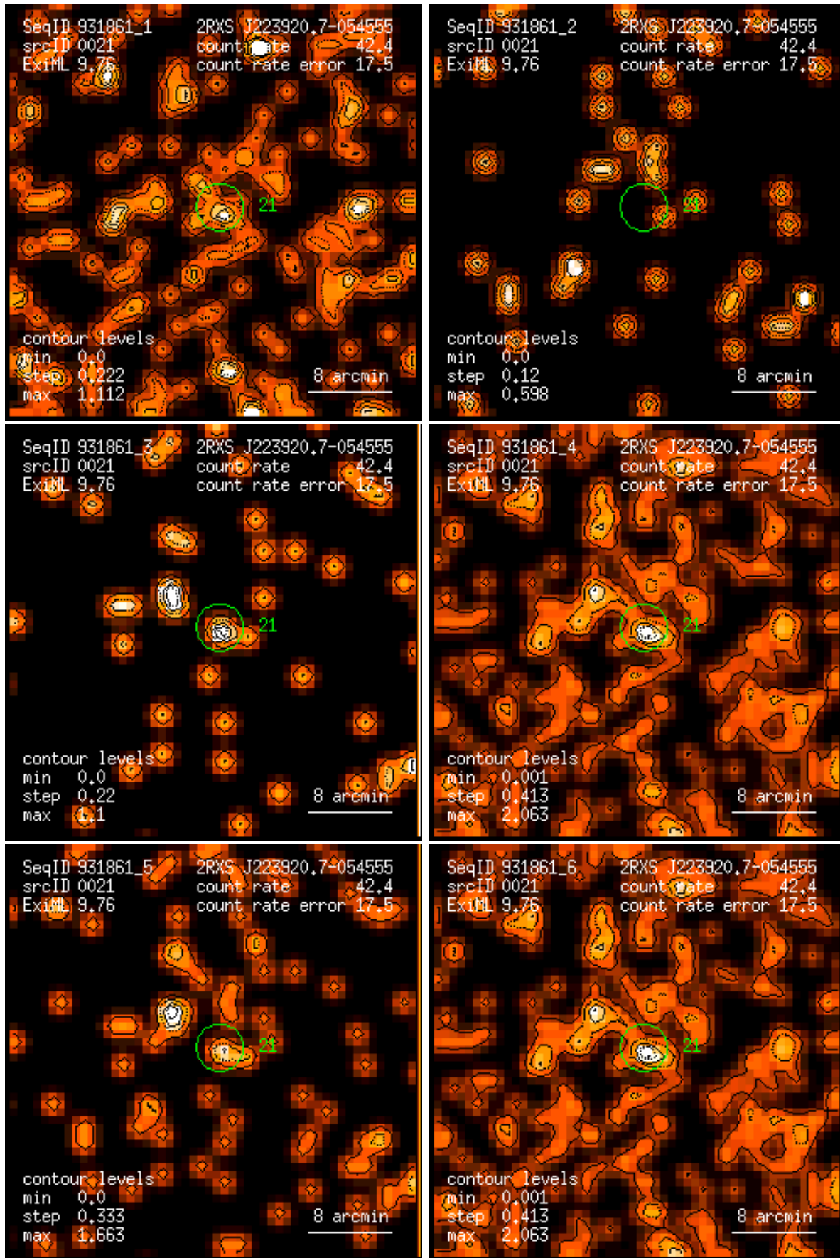
Figure 21: RASS 931861: detection 0021: band rate images, Gaussian filter: (1) PSPC channels 11 – 41, (2) 52 – 90, (3) 91 – 201, (4) 11 – 235, (5) 52 – 201, (6) 11 – 201. Broad band rates in counts/ks. Band rate contour levels in counts/ks/arcmin 2 .
