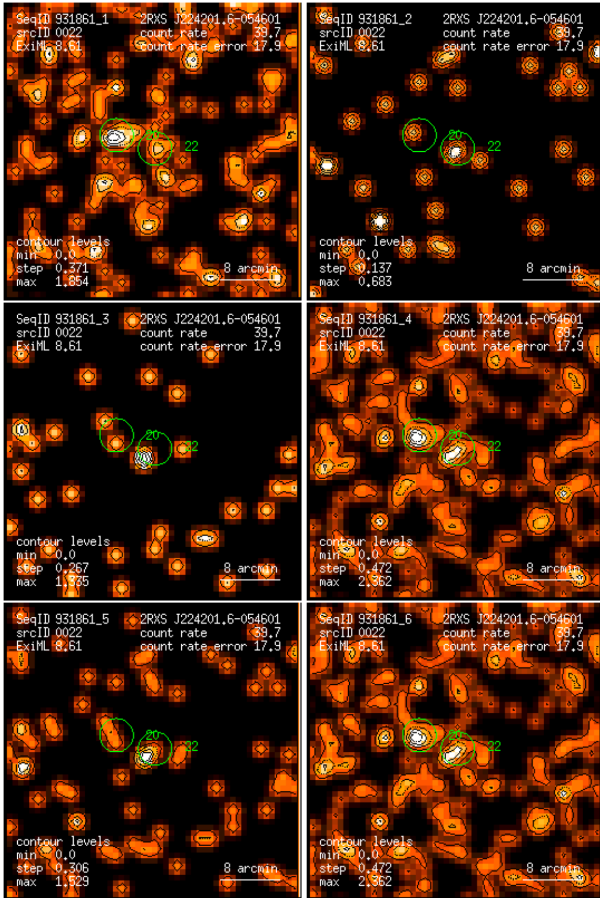
Figure 22: RASS 931861: detection 0022: band rate images, Gaussian filter: (1) PSPC channels 11 – 41, (2) 52 – 90, (3) 91 – 201, (4) 11 – 235, (5) 52 – 201, (6) 11 – 201. Broad band rates in counts/ks. Band rate contour levels in counts/ks/arcmin 2 .
