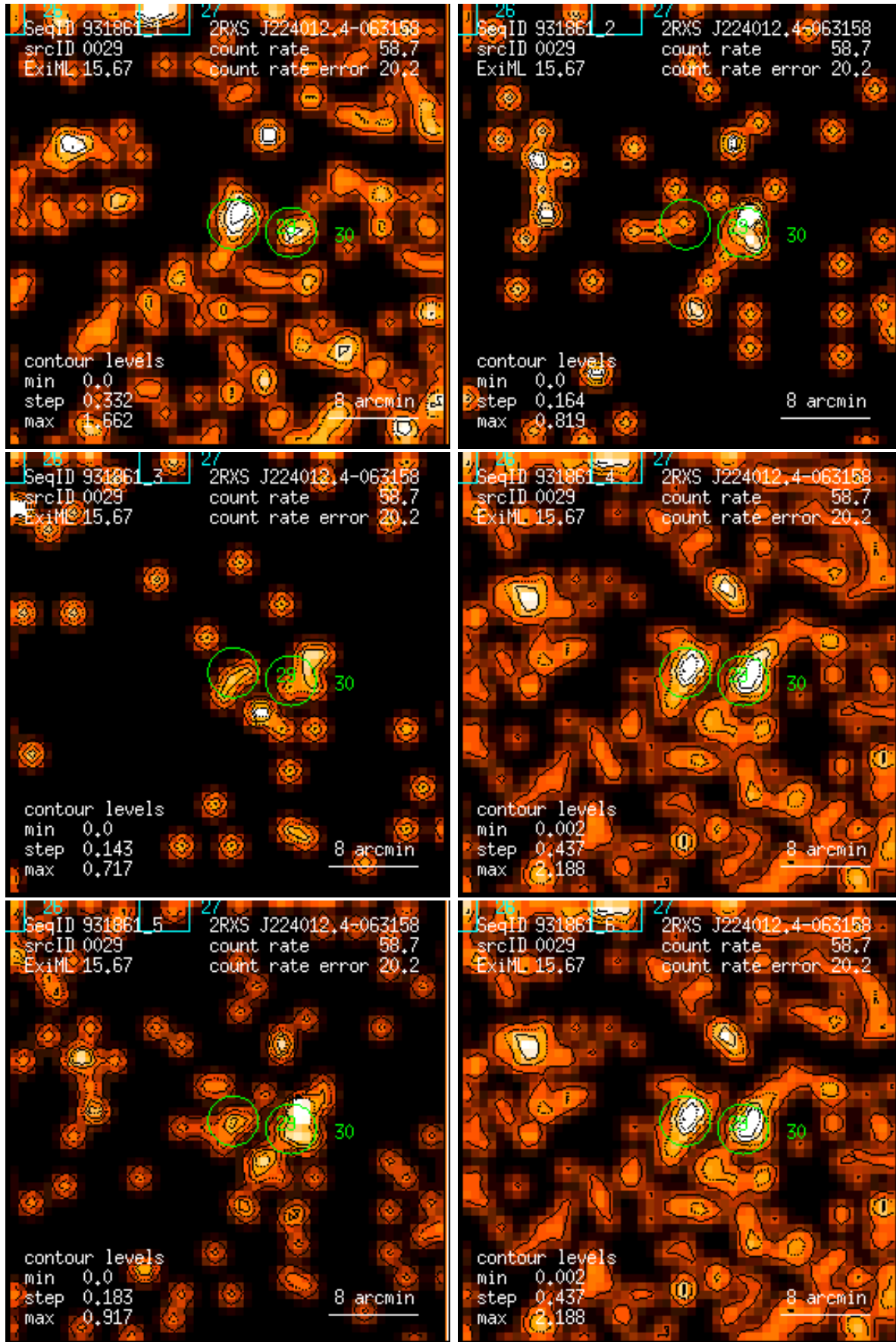
Figure 29: RASS 931861: detection 0029: band rate images, Gaussian filter: (1) PSPC channels 11 – 41, (2) 52 – 90, (3) 91 – 201, (4) 11 – 235, (5) 52 – 201, (6) 11 – 201. Broad band rates in counts/ks. Band rate contour levels in counts/ks/arcmin 2 .
