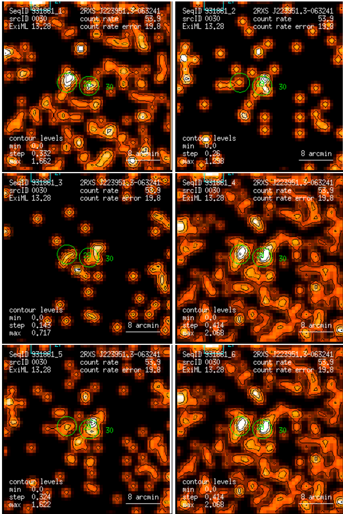
Figure 30: RASS 931861: detection 0030: band rate images, Gaussian filter: (1) PSPC channels 11 – 41, (2) 52 – 90, (3) 91 – 201, (4) 11 – 235, (5) 52 – 201, (6) 11 – 201. Broad band rates in counts/ks. Band rate contour levels in counts/ks/arcmin 2 .
