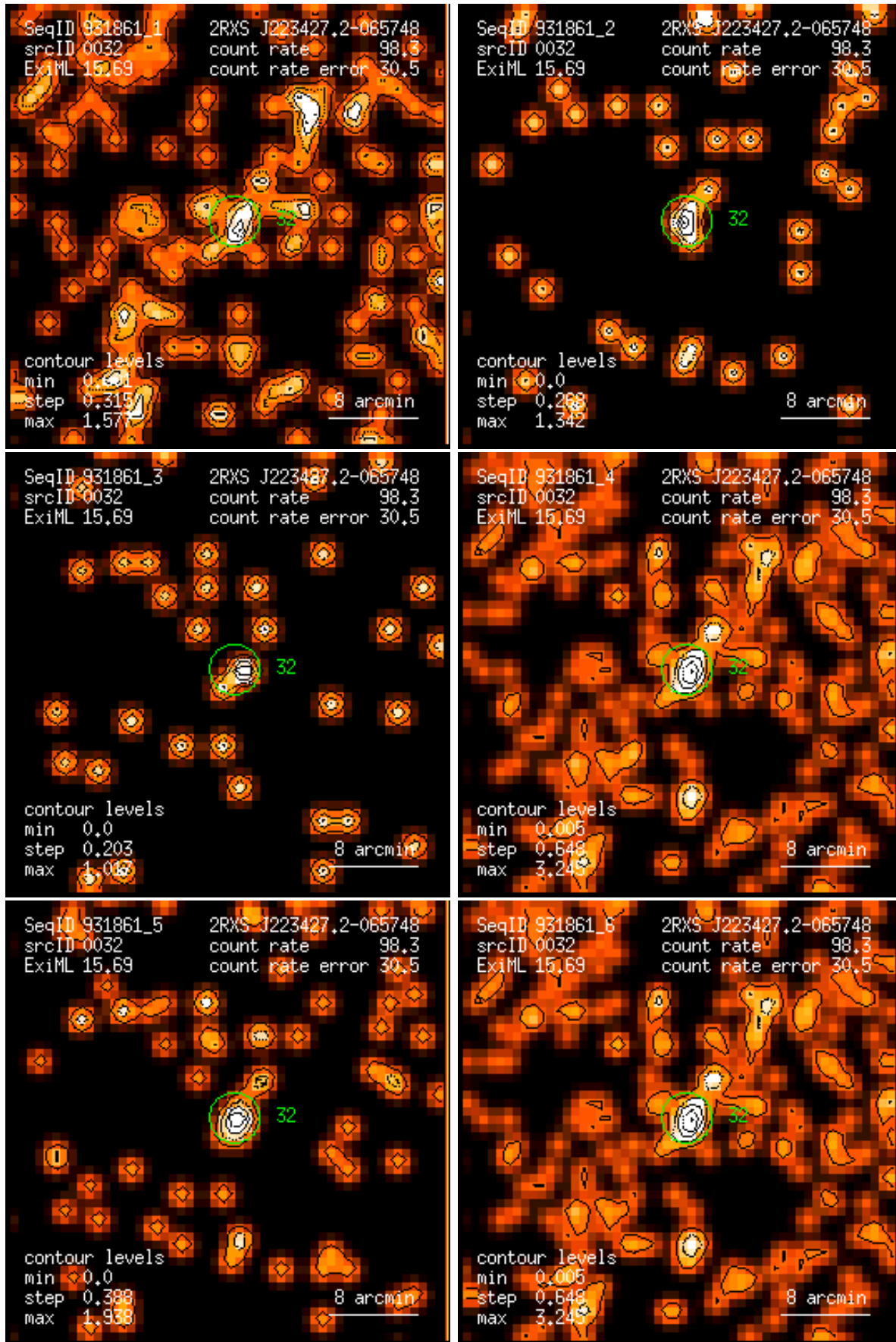
Figure 32: RASS 931861: detection 0032: band rate images, Gaussian filter: (1) PSPC channels 11 – 41, (2) 52 – 90, (3) 91 – 201, (4) 11 – 235, (5) 52 – 201, (6) 11 – 201. Broad band rates in counts/ks. Band rate contour levels in counts/ks/arcmin 2 .
