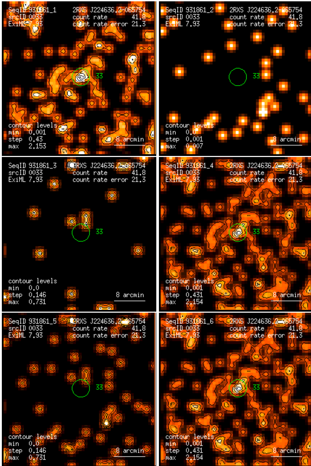
Figure 33: RASS 931861: detection 0033: band rate images, Gaussian filter: (1) PSPC channels 11 – 41, (2) 52 – 90, (3) 91 – 201, (4) 11 – 235, (5) 52 – 201, (6) 11 – 201. Broad band rates in counts/ks. Band rate contour levels in counts/ks/arcmin 2 .
