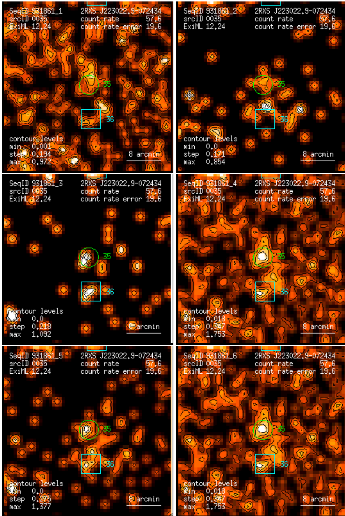
Figure 35: RASS 931861: detection 0035: band rate images, Gaussian filter: (1) PSPC channels 11 – 41, (2) 52 – 90, (3) 91 – 201, (4) 11 – 235, (5) 52 – 201, (6) 11 – 201. Broad band rates in counts/ks. Band rate contour levels in counts/ks/arcmin 2 .
