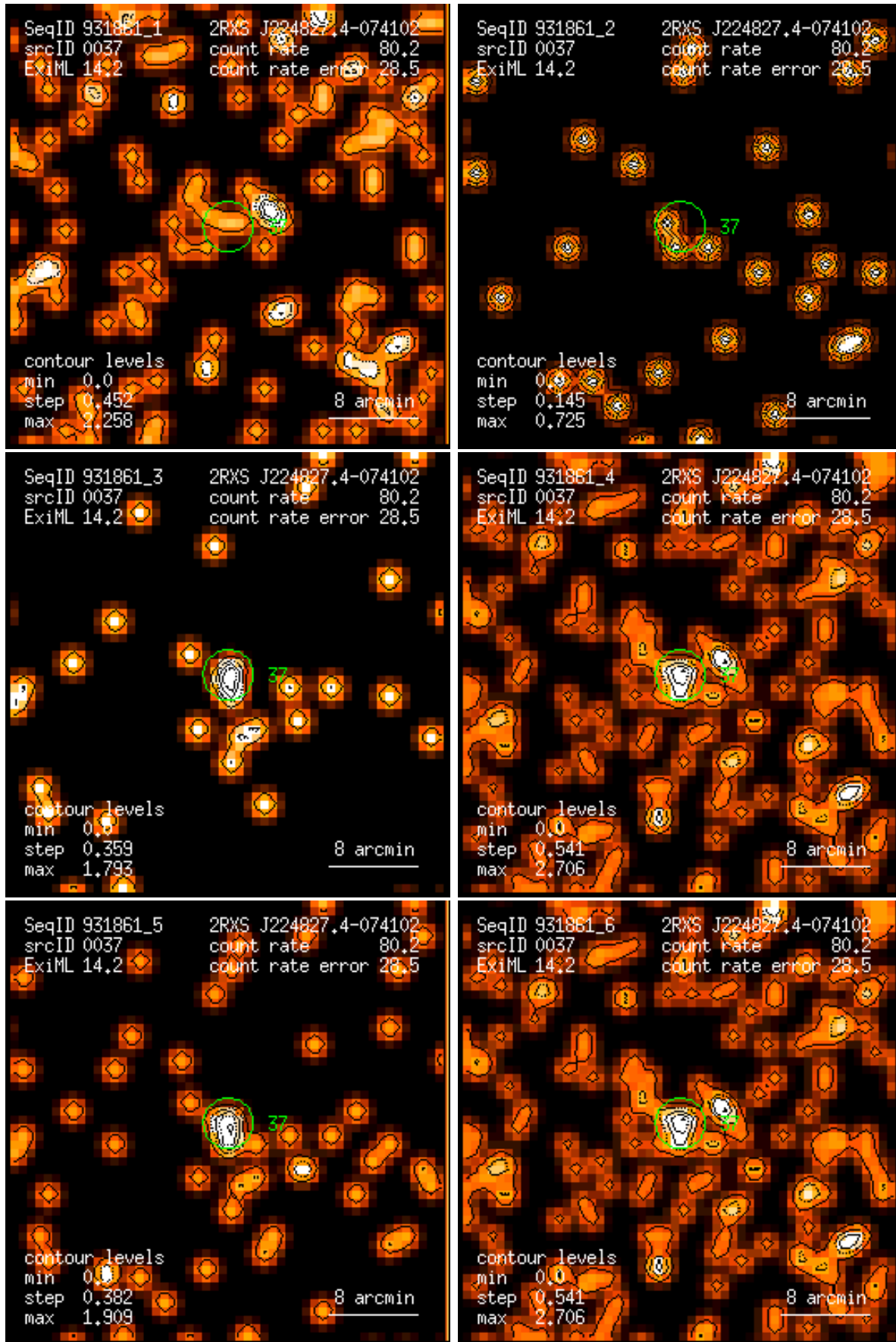
Figure 37: RASS 931861: detection 0037: band rate images, Gaussian filter: (1) PSPC channels 11 – 41, (2) 52 – 90, (3) 91 – 201, (4) 11 – 235, (5) 52 – 201, (6) 11 – 201. Broad band rates in counts/ks. Band rate contour levels in counts/ks/arcmin 2 .
