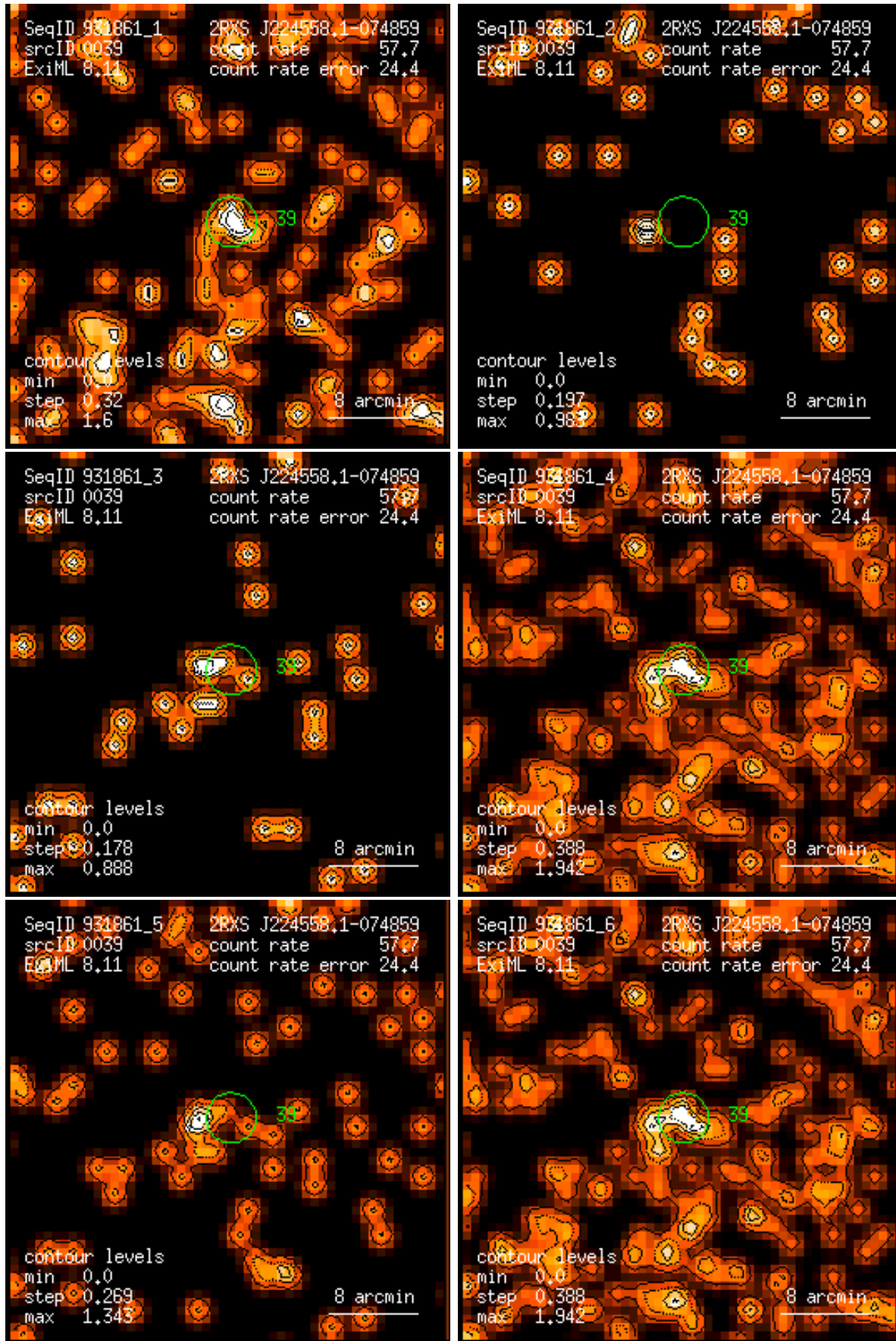
Figure 39: RASS 931861: detection 0039: band rate images, Gaussian filter: (1) PSPC channels 11 – 41, (2) 52 – 90, (3) 91 – 201, (4) 11 – 235, (5) 52 – 201, (6) 11 – 201. Broad band rates in counts/ks. Band rate contour levels in counts/ks/arcmin 2 .
