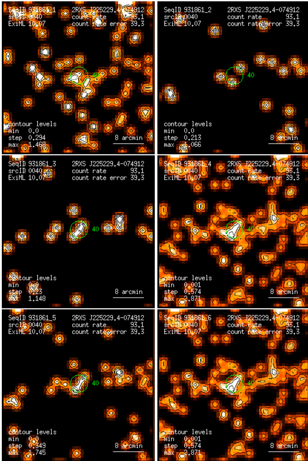
Figure 40: RASS 931861: detection 0040: band rate images, Gaussian filter: (1) PSPC channels 11 – 41, (2) 52 – 90, (3) 91 – 201, (4) 11 – 235, (5) 52 – 201, (6) 11 – 201. Broad band rates in counts/ks. Band rate contour levels in counts/ks/arcmin 2 .
