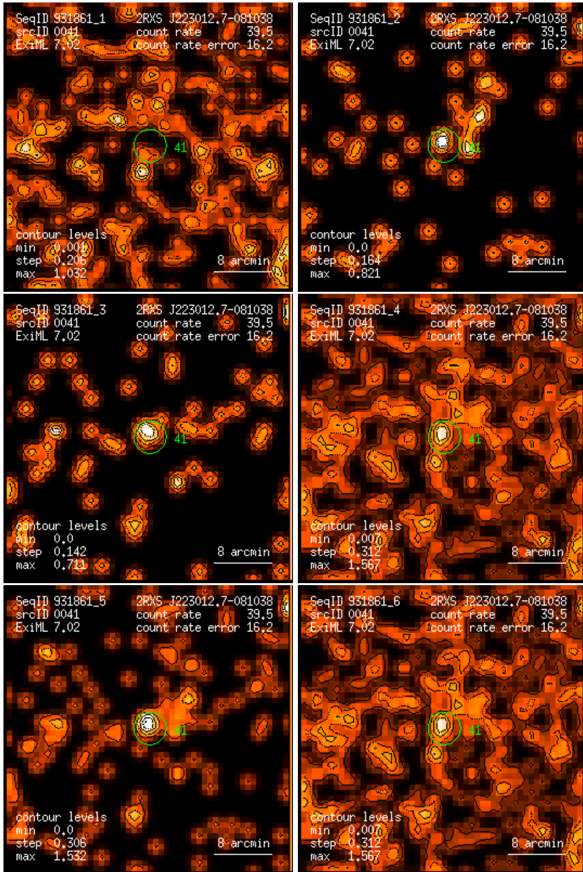
Figure 41: RASS 931861: detection 0041: band rate images, Gaussian filter: (1) PSPC channels 11 – 41, (2) 52 – 90, (3) 91 – 201, (4) 11 – 235, (5) 52 – 201, (6) 11 – 201. Broad band rates in counts/ks. Band rate contour levels in counts/ks/arcmin 2 .
