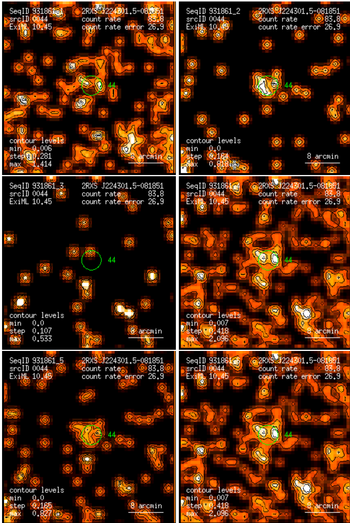
Figure 44: RASS 931861: detection 0044: band rate images, Gaussian filter: (1) PSPC channels 11 – 41, (2) 52 – 90, (3) 91 – 201, (4) 11 – 235, (5) 52 – 201, (6) 11 – 201. Broad band rates in counts/ks. Band rate contour levels in counts/ks/arcmin 2 .
