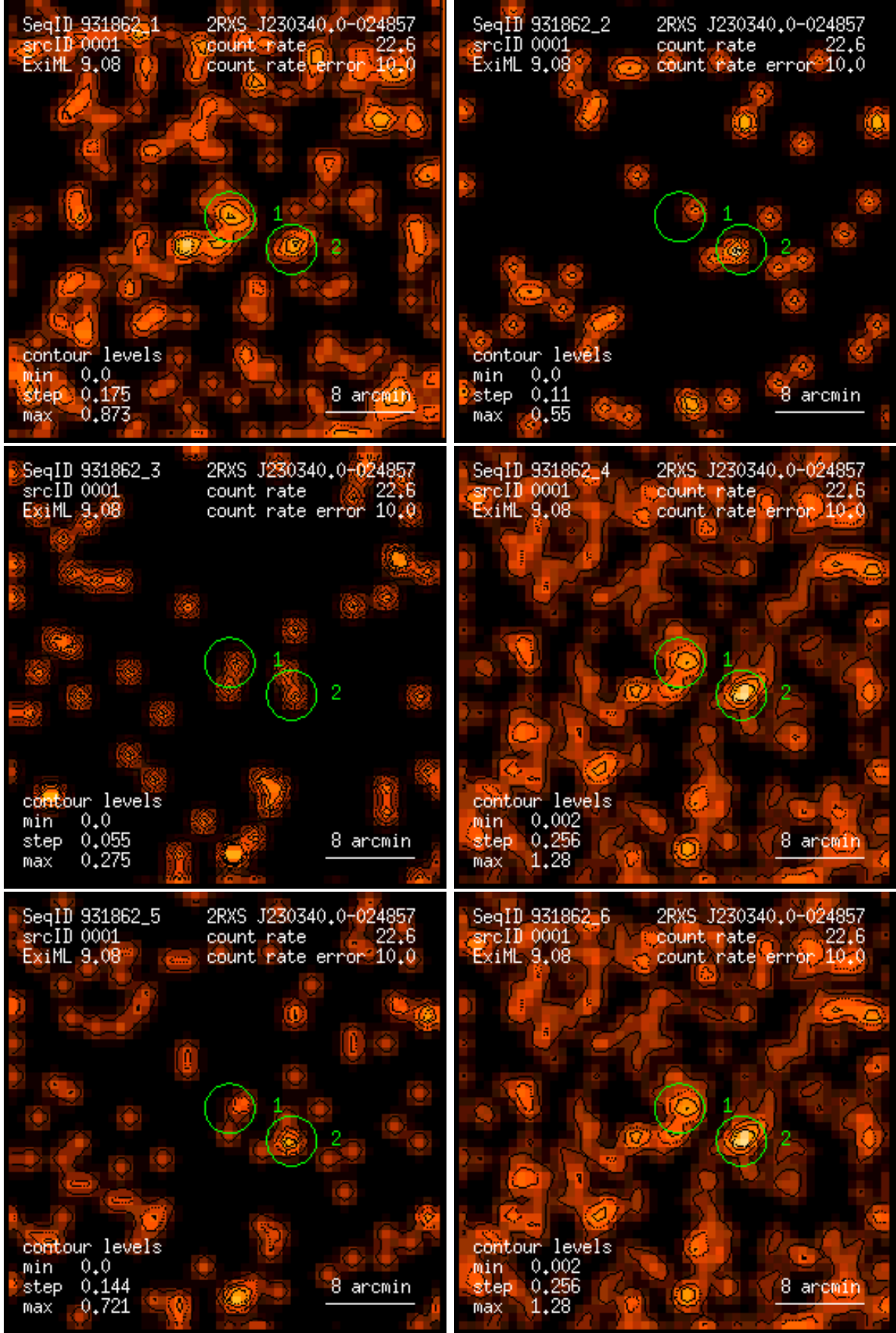
Figure 1: RASS 931862: detection 0001: band rate images, Gaussian filter: (1) PSPC channels 11 – 41, (2) 52 – 90, (3) 91 – 201, (4) 11 – 235, (5) 52 – 201, (6) 11 – 201. Broad band rates in counts/ks. Band rate contour levels in counts/ks/arcmin 2 .
