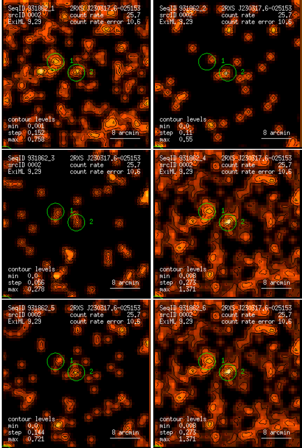
Figure 2: RASS 931862: detection 0002: band rate images, Gaussian filter: (1) PSPC channels 11 – 41, (2) 52 – 90, (3) 91 – 201, (4) 11 – 235, (5) 52 – 201, (6) 11 – 201. Broad band rates in counts/ks. Band rate contour levels in counts/ks/arcmin 2 .
