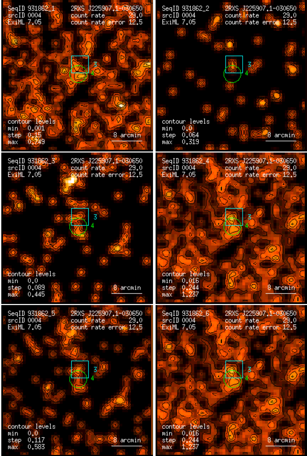
Figure 4: RASS 931862: detection 0004: band rate images, Gaussian filter: (1) PSPC channels 11 – 41, (2) 52 – 90, (3) 91 – 201, (4) 11 – 235, (5) 52 – 201, (6) 11 – 201. Broad band rates in counts/ks. Band rate contour levels in counts/ks/arcmin 2 .
