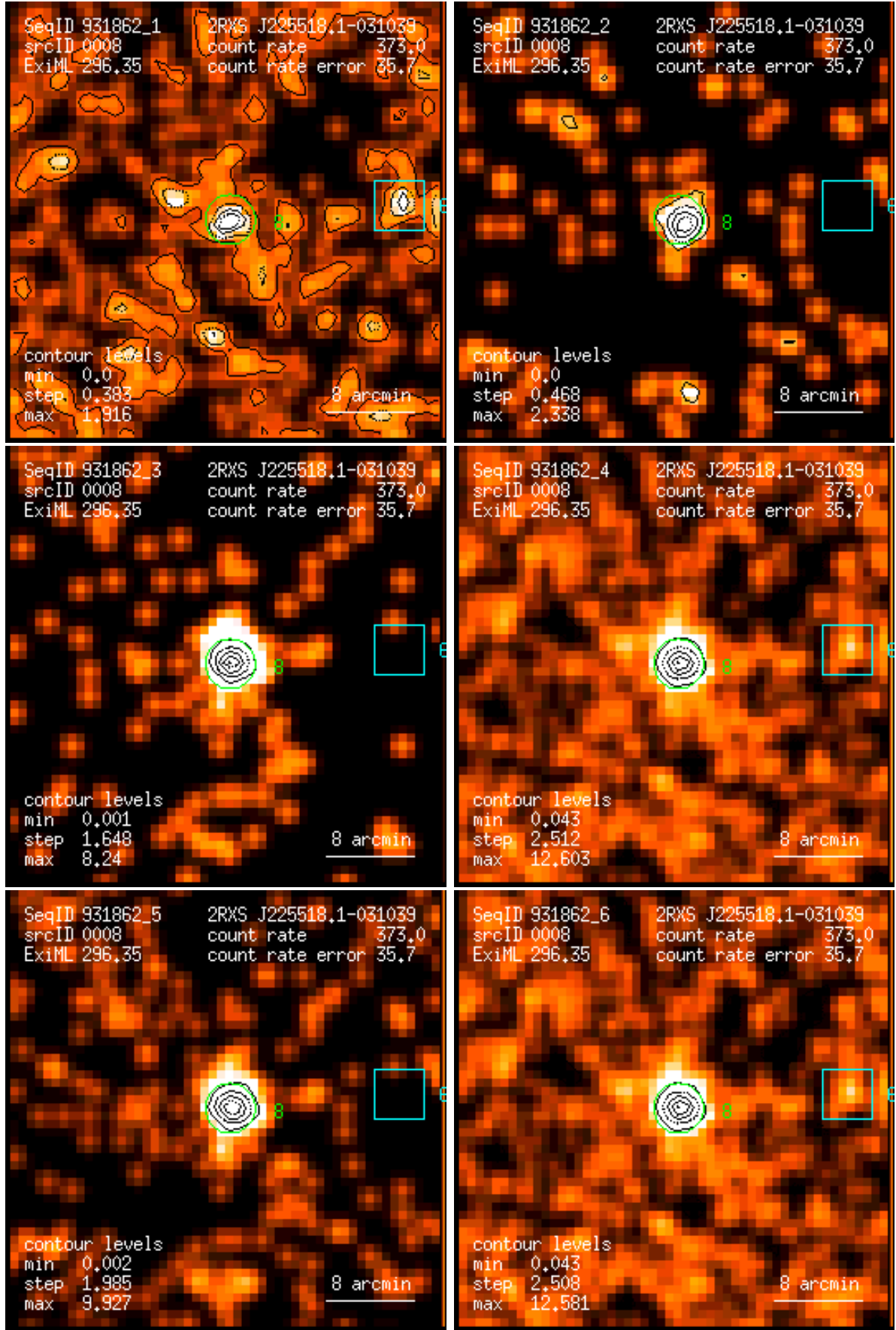
Figure 8: RASS 931862: detection 0008: band rate images, Gaussian filter: (1) PSPC channels 11 – 41, (2) 52 – 90, (3) 91 – 201, (4) 11 – 235, (5) 52 – 201, (6) 11 – 201. Broad band rates in counts/ks. Band rate contour levels in counts/ks/arcmin 2 .
