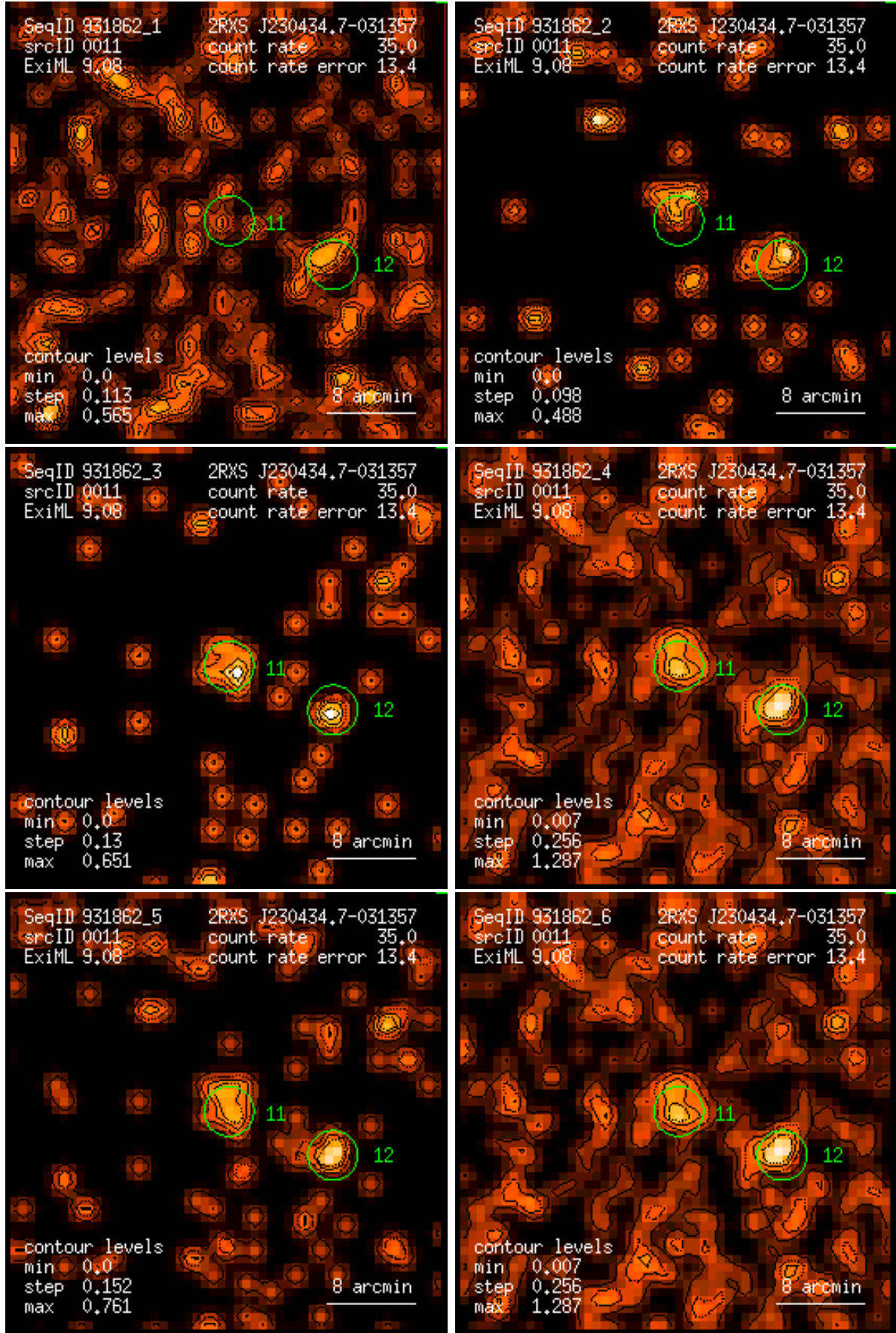
Figure 11: RASS 931862: detection 0011: band rate images, Gaussian filter: (1) PSPC channels 11 – 41, (2) 52 – 90, (3) 91 – 201, (4) 11 – 235, (5) 52 – 201, (6) 11 – 201. Broad band rates in counts/ks. Band rate contour levels in counts/ks/arcmin 2 .
