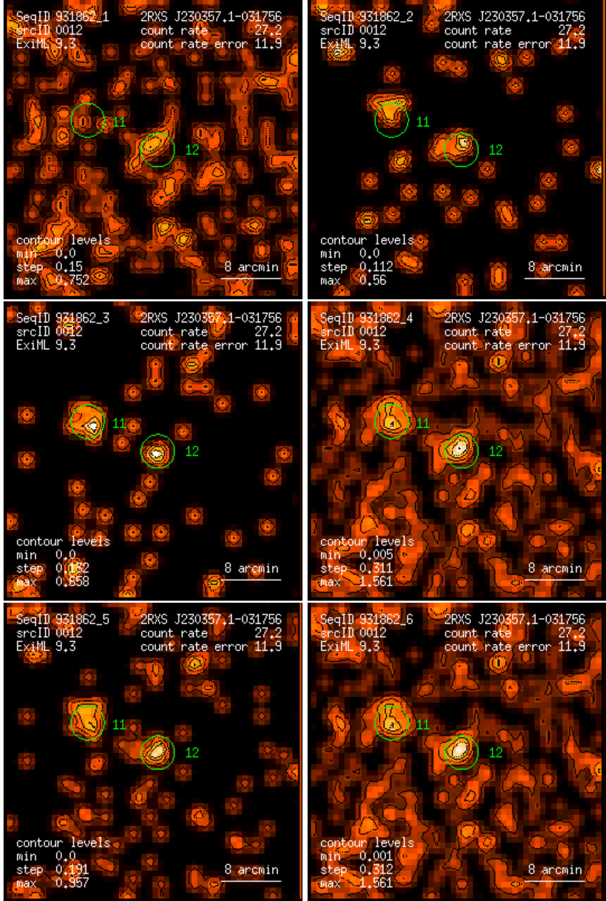
Figure 12: RASS 931862: detection 0012: band rate images, Gaussian filter: (1) PSPC channels 11 – 41, (2) 52 – 90, (3) 91 – 201, (4) 11 – 235, (5) 52 – 201, (6) 11 – 201. Broad band rates in counts/ks. Band rate contour levels in counts/ks/arcmin 2 .
