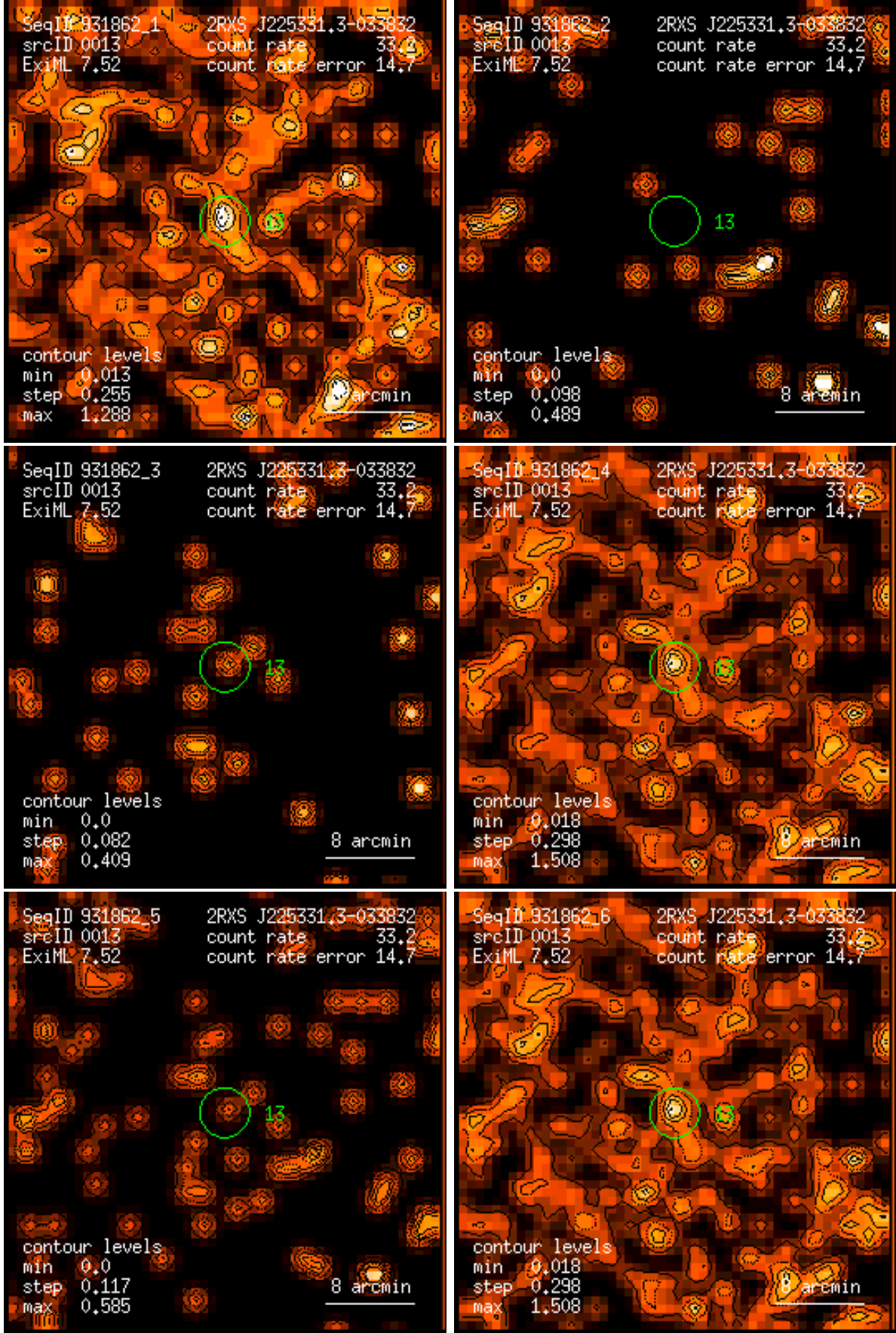
Figure 13: RASS 931862: detection 0013: band rate images, Gaussian filter: (1) PSPC channels 11 – 41, (2) 52 – 90, (3) 91 – 201, (4) 11 – 235, (5) 52 – 201, (6) 11 – 201. Broad band rates in counts/ks. Band rate contour levels in counts/ks/arcmin 2 .
