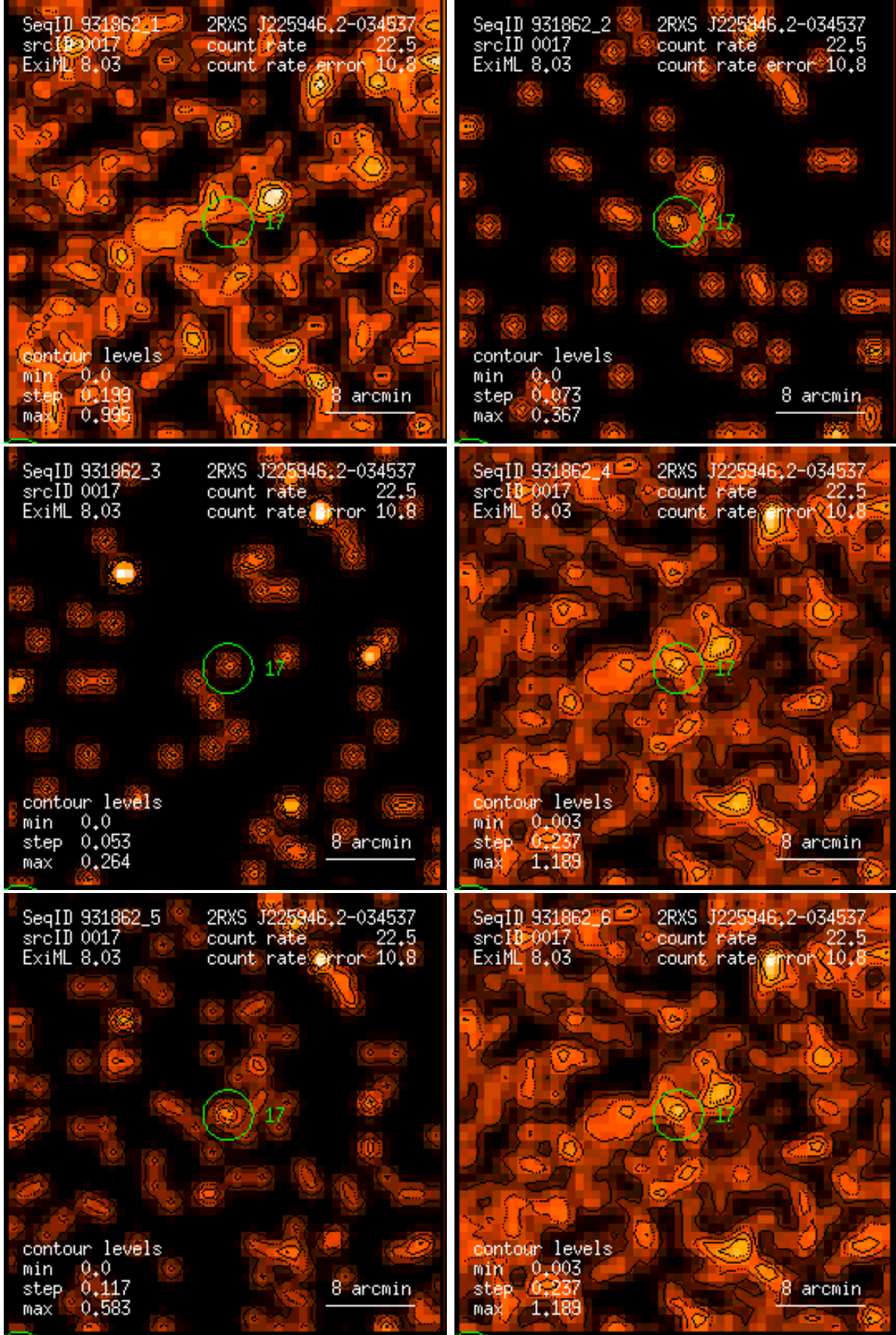
Figure 17: RASS 931862: detection 0017: band rate images, Gaussian filter: (1) PSPC channels 11 – 41, (2) 52 – 90, (3) 91 – 201, (4) 11 – 235, (5) 52 – 201, (6) 11 – 201. Broad band rates in counts/ks. Band rate contour levels in counts/ks/arcmin 2 .
