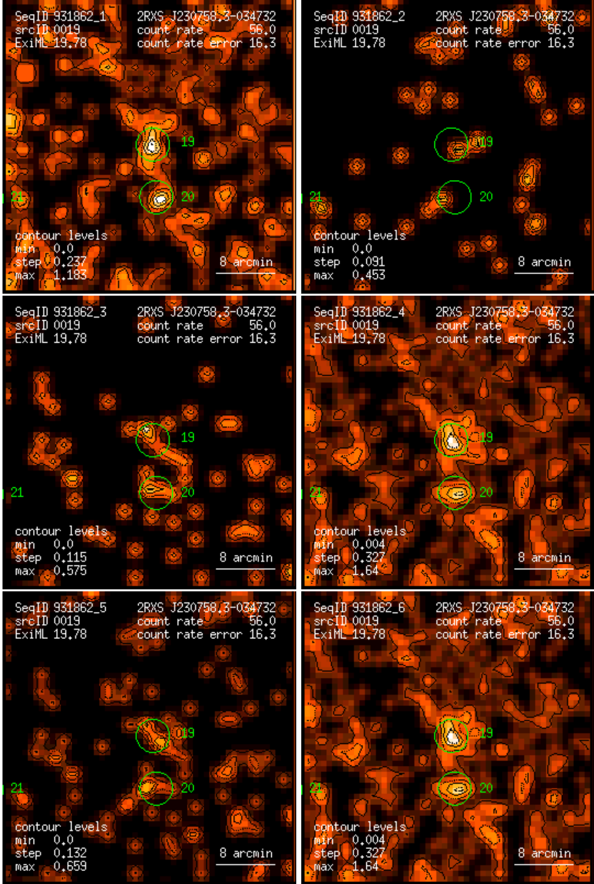
Figure 19: RASS 931862: detection 0019: band rate images, Gaussian filter: (1) PSPC channels 11 – 41, (2) 52 – 90, (3) 91 – 201, (4) 11 – 235, (5) 52 – 201, (6) 11 – 201. Broad band rates in counts/ks. Band rate contour levels in counts/ks/arcmin 2 .
