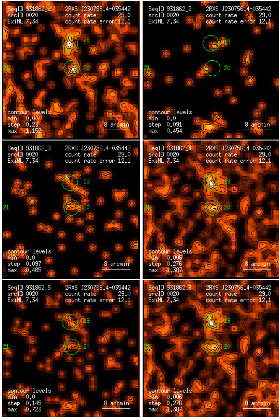
Figure 20: RASS 931862: detection 0020: band rate images, Gaussian filter: (1) PSPC channels 11 – 41, (2) 52 – 90, (3) 91 – 201, (4) 11 – 235, (5) 52 – 201, (6) 11 – 201. Broad band rates in counts/ks. Band rate contour levels in counts/ks/arcmin 2 .
