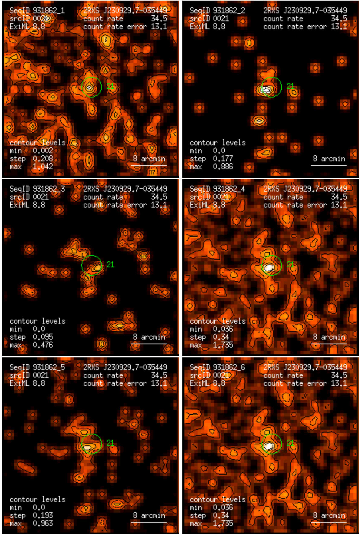
Figure 21: RASS 931862: detection 0021: band rate images, Gaussian filter: (1) PSPC channels 11 – 41, (2) 52 – 90, (3) 91 – 201, (4) 11 – 235, (5) 52 – 201, (6) 11 – 201. Broad band rates in counts/ks. Band rate contour levels in counts/ks/arcmin 2 .
