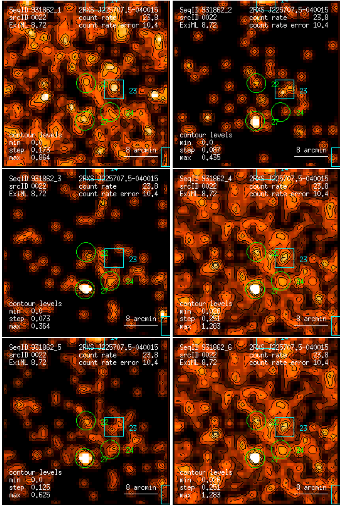
Figure 22: RASS 931862: detection 0022: band rate images, Gaussian filter: (1) PSPC channels 11 – 41, (2) 52 – 90, (3) 91 – 201, (4) 11 – 235, (5) 52 – 201, (6) 11 – 201. Broad band rates in counts/ks. Band rate contour levels in counts/ks/arcmin 2 .
